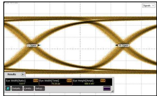
Figure 26. TL = 3-Meter 30-AWG 100 \Omega Twin-Axial Cable, DS100BR111A CHA, 10.3125 Gbps
