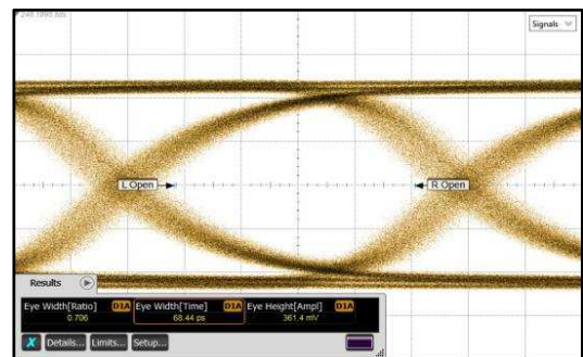
Figure 28. TL = 7-Meter 30-AWG 100 \Omega Twin-Axial Cable, DS100BR111A CHA, 10.3125 Gbps
