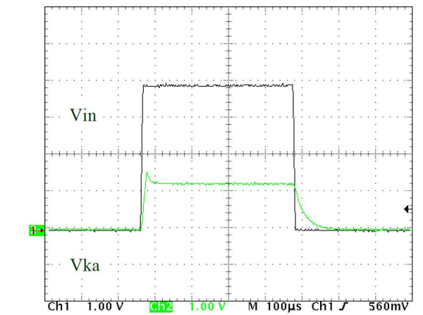
Figure 13. Turn-on ( C_{LOAD} = 10 \text{ nF} )
