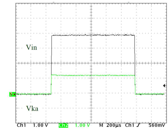
Figure 12. Turn-on (no C_{LOAD} )
