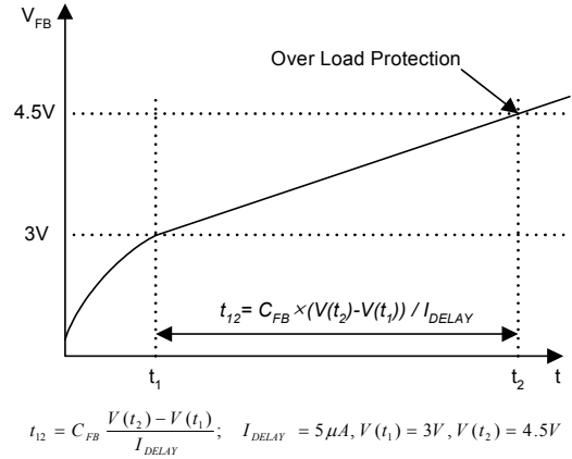
Figure 10. Over Load Protection (OLP)
