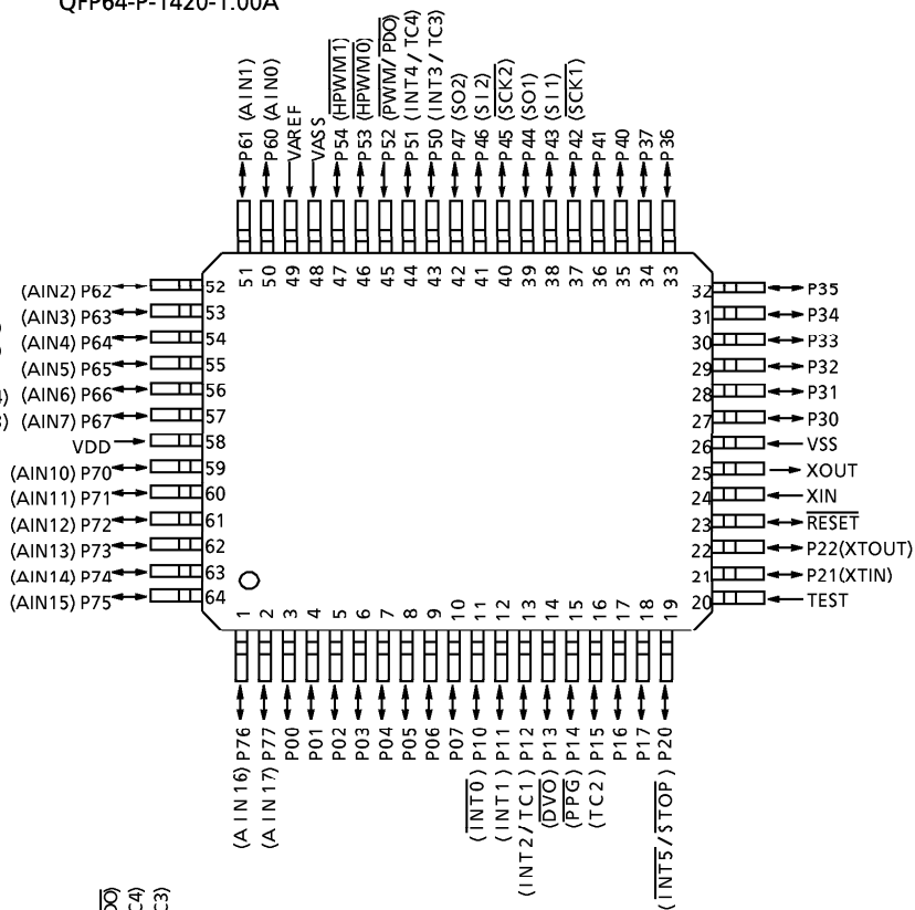
QFP64-P-1420-1.00A
