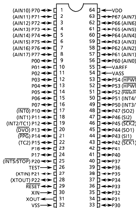
SDIP64-P-750-1.78
