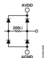
Figure 7. VIN+, VIN-
