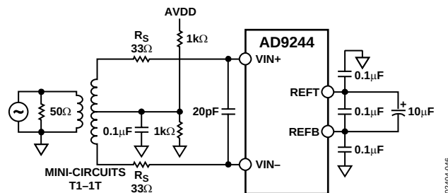
Figure 46. Transformer-Coupled Input
