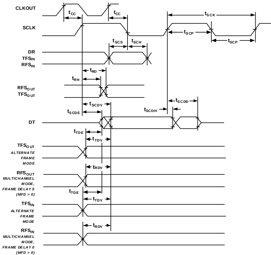
Figure 21. Serial Ports
