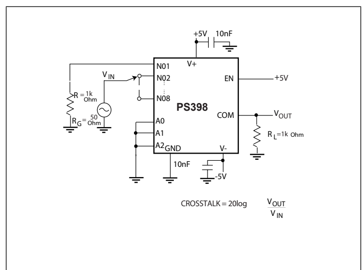
Figure 6. CrossTalk
