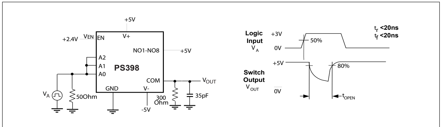
Figure 3. Break-Before-Make Interval
