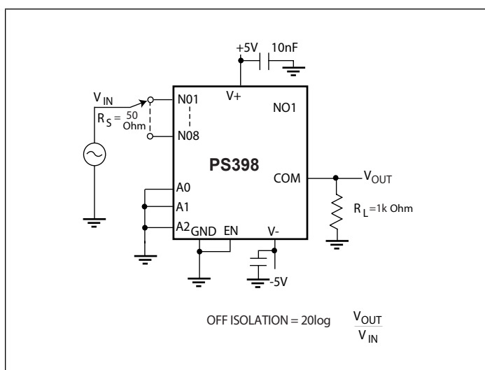
Figure 5. Off Isolation
