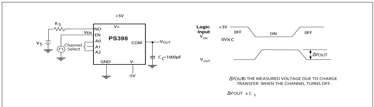
Figure 4. Charge Injection
