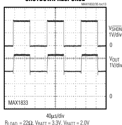
SHUTDOWN RESPONSE
