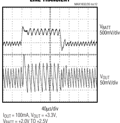
LINE TRANSIENT
