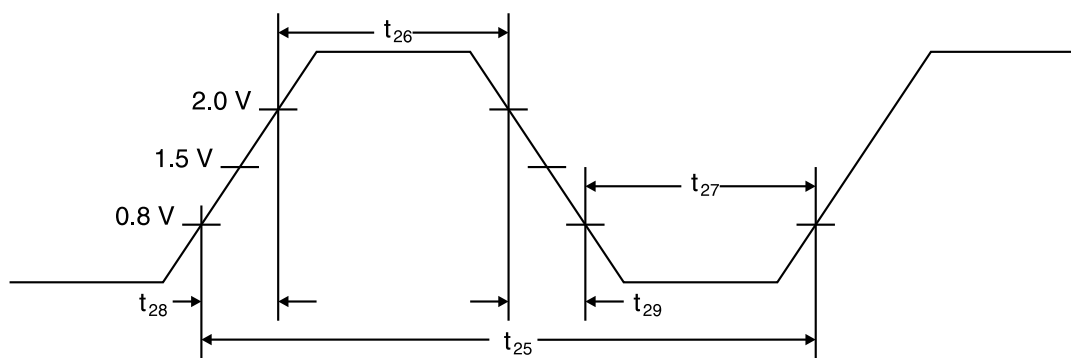
Figure 45. TCK Waveforms
