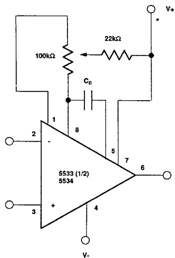
Frequency Compensation and Offset Voltage Adjustment Circuit
