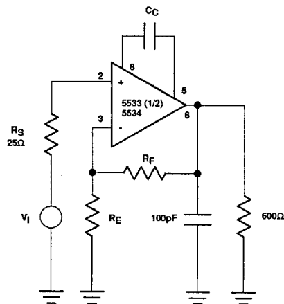
Closed-Loop Frequency Response
