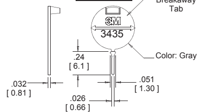
3435-0 Keying Plug (Optional: Order Separately) Material: Gray Polyester (PBT)
