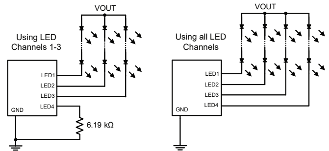
Figure 6: How to signal an unused LED channel during startup LED detection phase
