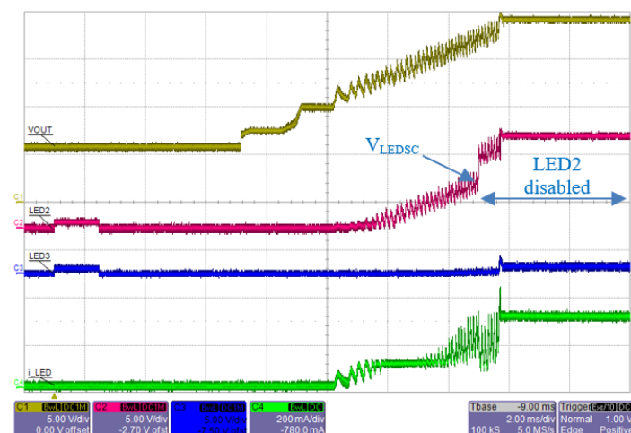
Figure 35: Startup sequence when LED string#2 has a partial-short fault ( 4 \times \text{WLED} instead of 6). As soon as LED2 pin rises above V_{LEDSC} ( \sim 4.6\text{ V} ), the channel is disabled. Output is now 300\text{ mA} .
