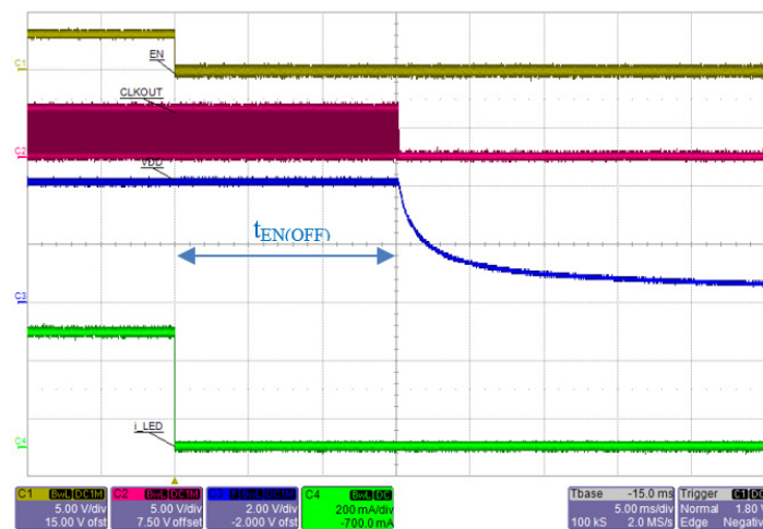
Figure 32: After EN = L for 32k clock cycles (~15 ms at 2.15 MHz), the IC completely shuts down so VDD (Blue) decays.
