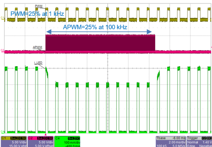
Figure 27: PWM = 25\% at 1\text{ kHz} . Peak LED current drops from 400\text{ mA} ( 4 \times 100\text{ mA/ch} ) to 300\text{ mA} when APWM of 25\% duty cycle is applied
