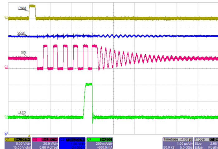
Figure 20: Zoom-in view showing ALT80600 is able to regulate LED current at PWM on-time down to 300 ns.
