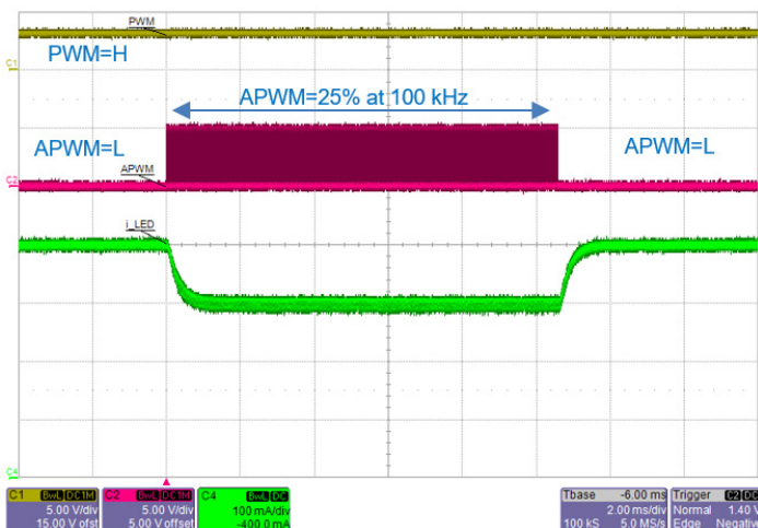
Figure 26: PWM = H. Total LED current drops from 400\text{ mA} ( 4 \times 100\text{ mA/ch} ) to 300\text{ mA} when APWM of 25\% duty cycle is applied. Note that LED current takes \sim 0.5\text{ ms} to settle after change in APWM.
