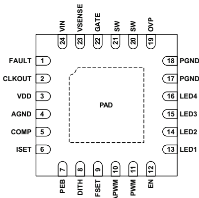
Package ES, 24-Pin QFN Pinouts
