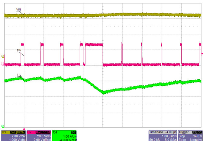
Figure 39: When peak current in SW pin reaches ~3.2 A, overcurrent protection kicks in and the IC skips a switching cycle.
