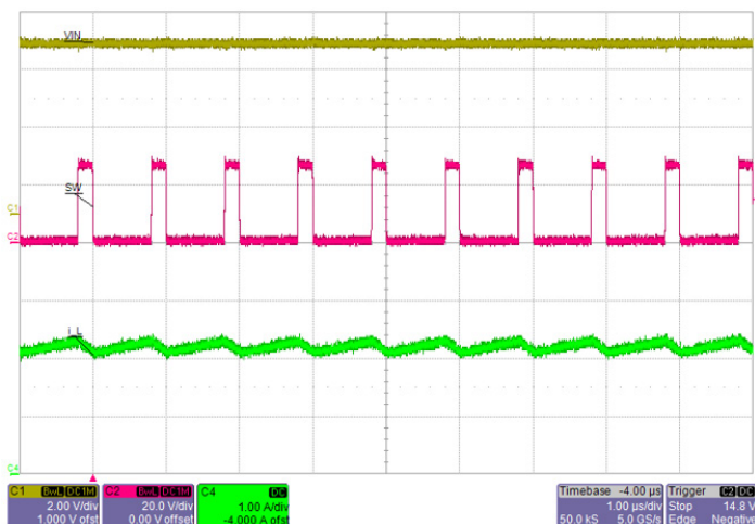
Figure 38: Normal switching waveform showing the SW node voltage and inductor current.
