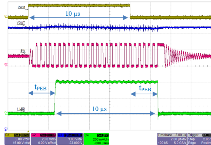
Figure 19: Zoom in view for PWM on-time = 10 \mu s. Notice that the LED current is shifted with respect to PWM signal. Ripple at V_{OUT} is ~0.2 V when using 2 \times 4.7 \mu F MLCC as output capacitors.
