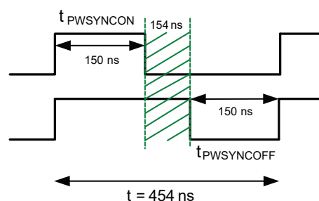
Figure 13: Pulse width requirements for an External Sync clock at 2.2 MHz
