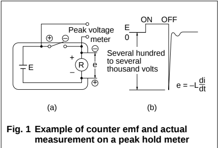
Fig. 1 Example of counter emf and actual measurement on a peak hold meter
