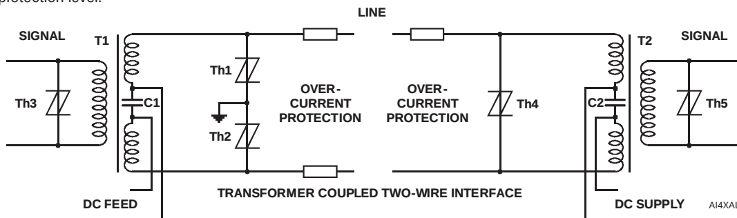
Figure 11. 2-Wire System
