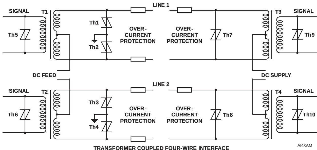
Figure 12. 4-Wire System
