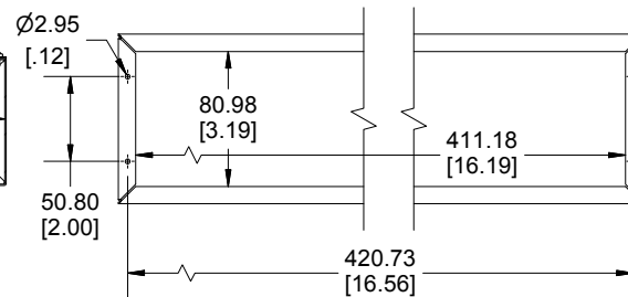
Bottom View of Chassis (Sold Separately)
