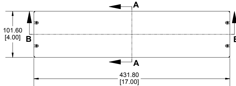
Bottom View of Assembly
