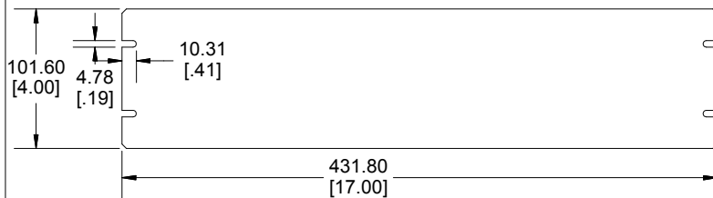
Bottom Plate (Sold Separately)
