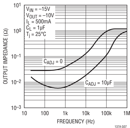
Output Impedance
