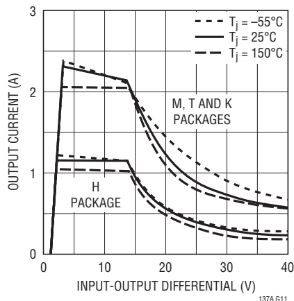
Current Limit
