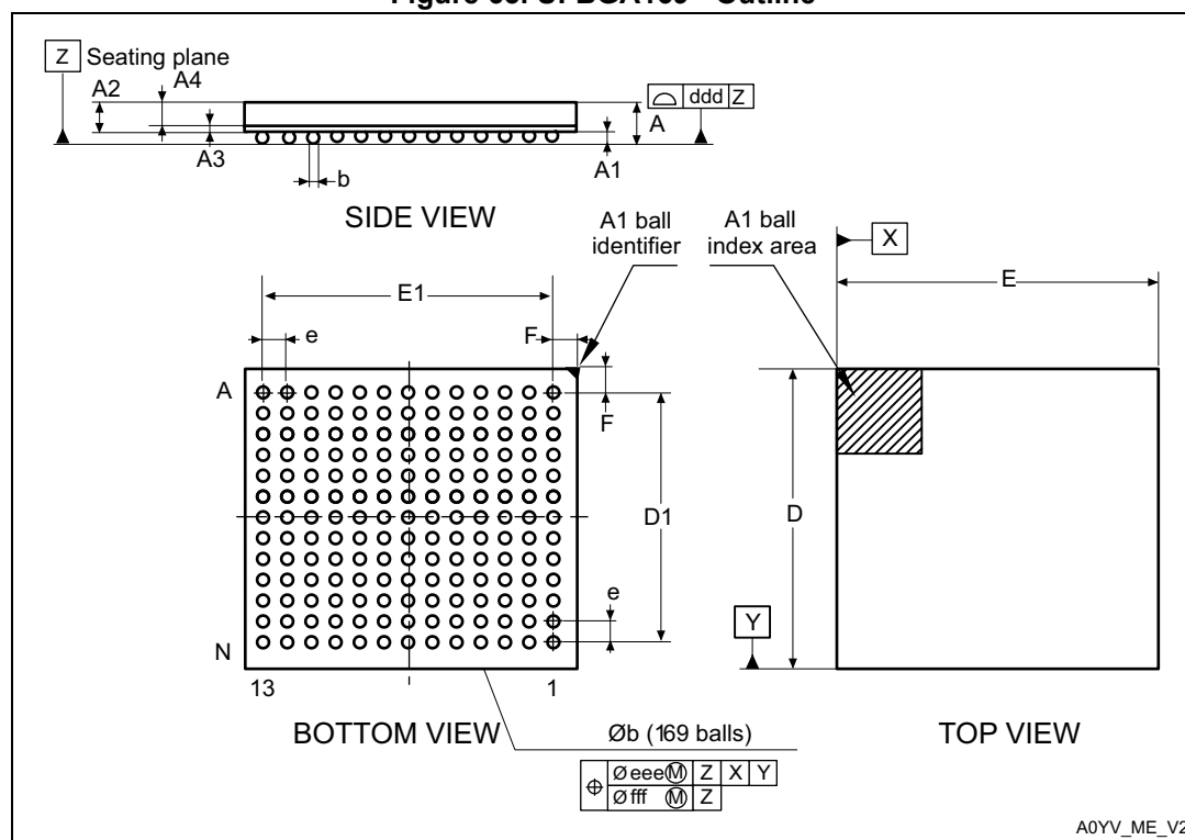
Figure 63. UFBGA169 - Outline
