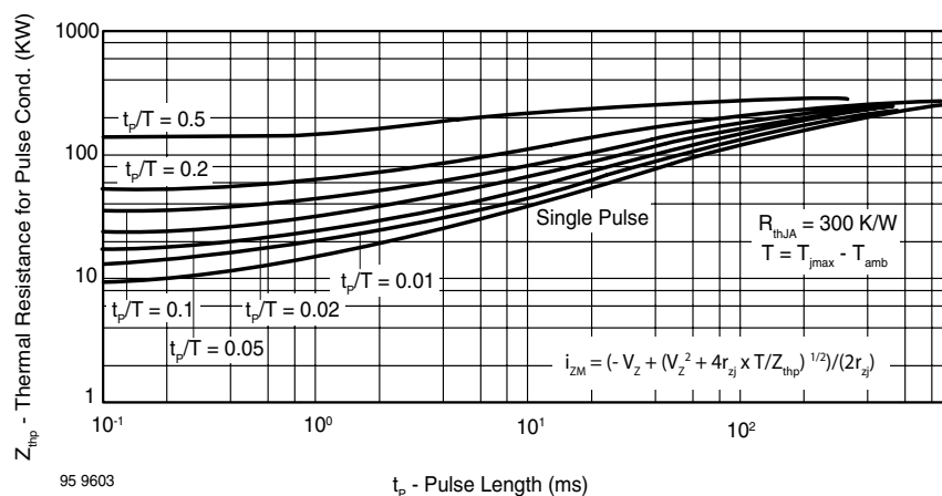
Figure 11. Thermal Response
