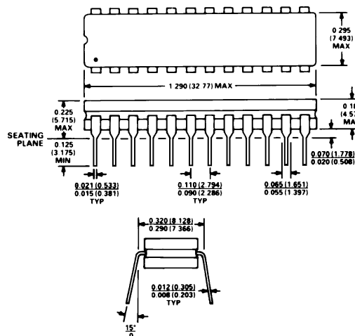
24-Pin Cerdip (Q-24)
