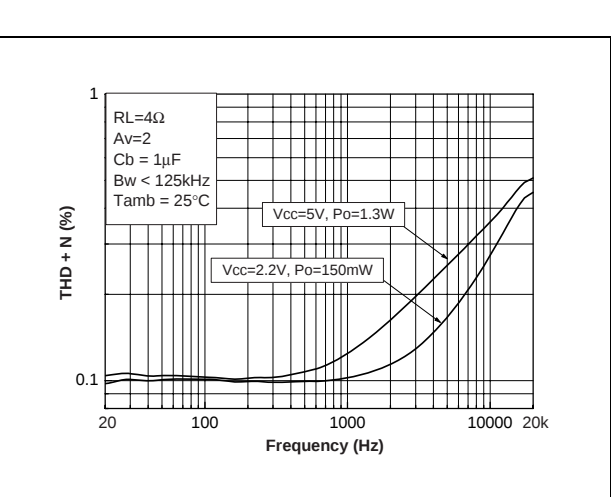
Figure 53. THD + N vs. frequency
