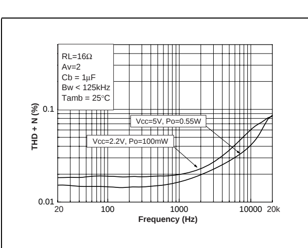
Figure 54. THD + N vs. frequency
