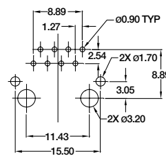
RECOMMENDED PC BOARD LAYOUT (TOP VIEW) SHIELD OPTION 04
