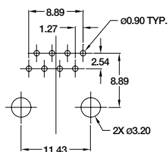
RECOMMENDED PC BOARD LAYOUT (TOP VIEW)
