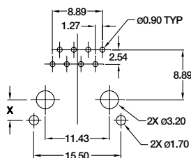
RECOMMENDED PC BOARD LAYOUT (TOP VIEW) SHIELD OPTION 02, 03
