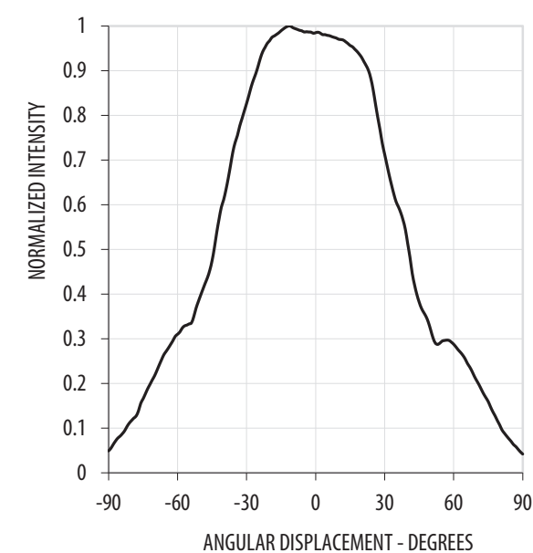
Figure 5: Radiation Pattern
