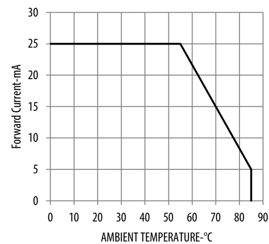
Figure 10: Derating Curve
