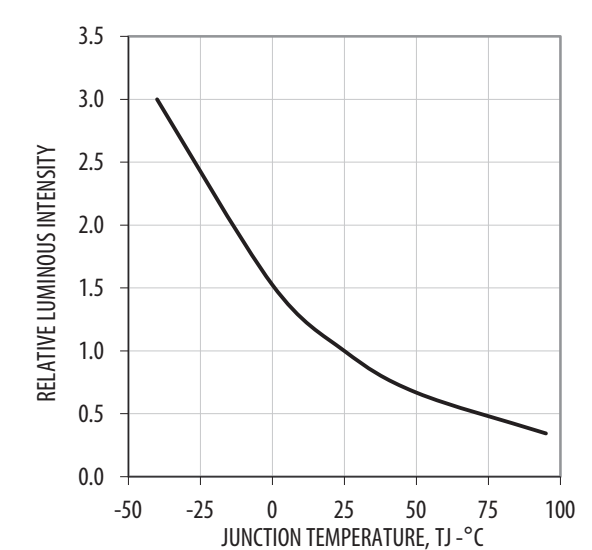
Figure 7: Relative Intensity vs. Temperature
