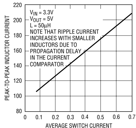
Peak-to-Peak Inductor Ripple Current
