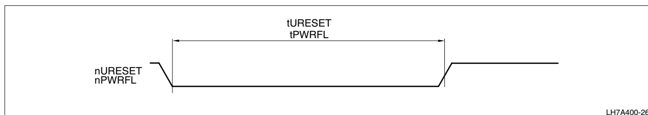
Figure 43. External Reset
