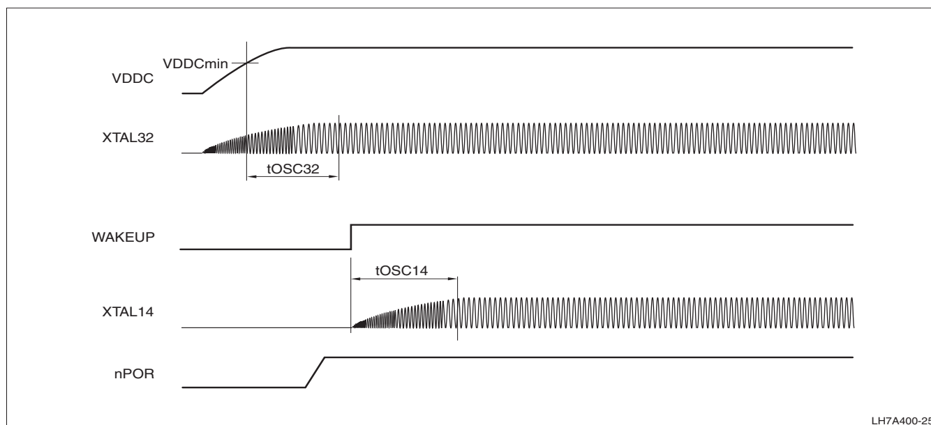
Figure 42. Oscillator Start-up
