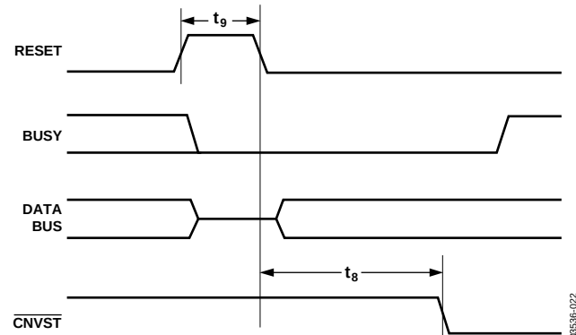
Figure 23. Reset Timing
