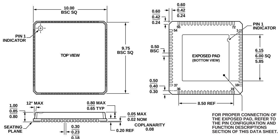
Figure 5. 72-Lead Lead Frame Chip Scale Package [LFCSP_VQ]
