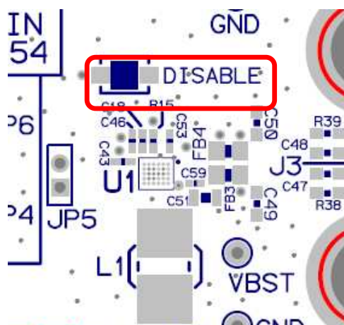
Figure 4. DISABLE Pushbutton
