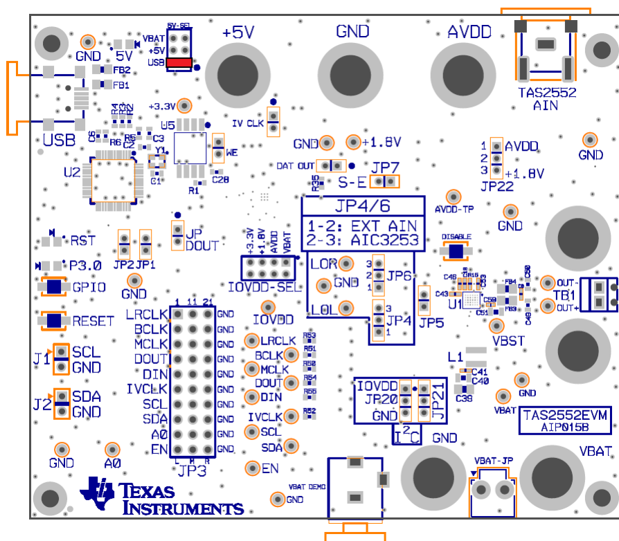
Figure 1. Power Connections
