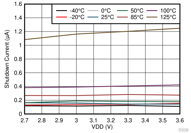
Figure 5-7. Shutdown Mode I_{DD} vs V_{DD}
