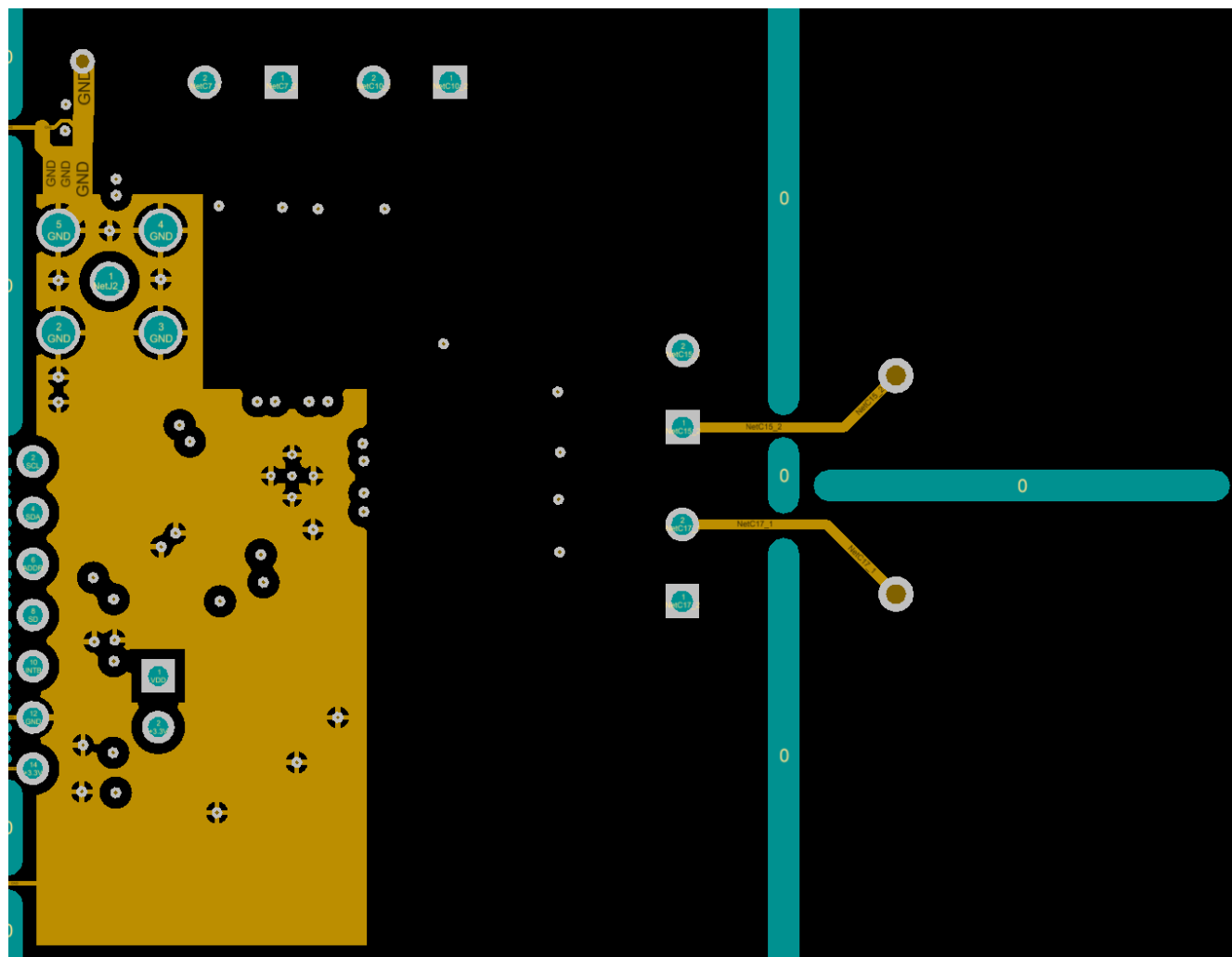
Figure 7-10. Example PCB Layout: Mid-Layer 1 (GND)
