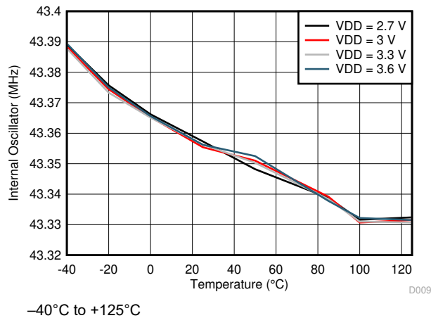
Figure 5-8. Internal Oscillator Frequency vs Temperature
