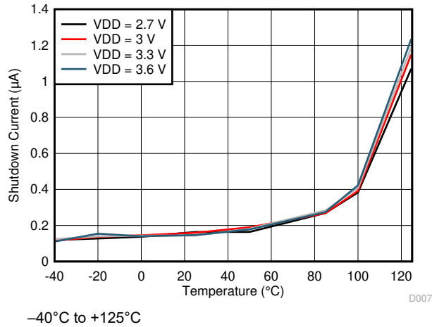
Figure 5-6. Shutdown Mode I_{DD} vs Temperature
