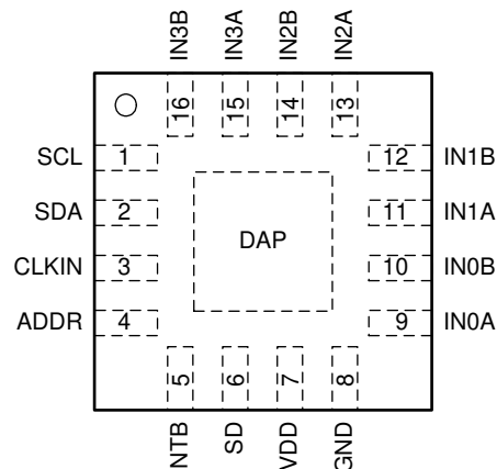
Figure 4-2. FDC2114/FDC2214 RGH Package 16-Pin WQFN Top View
