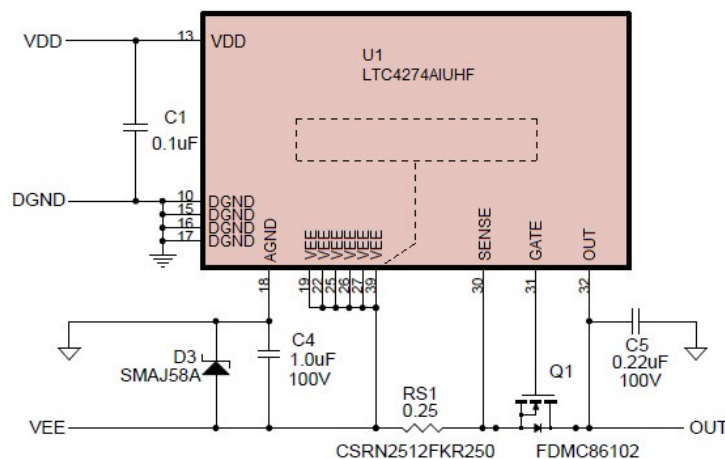
Figure 2. LTC4274A Key Application Components for Board Placement
