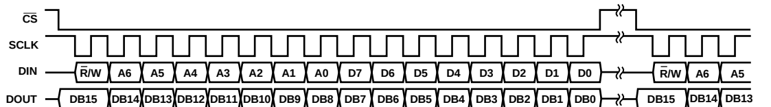
Figure 11. Example SPI Read, Second 16-Bit Sequence
