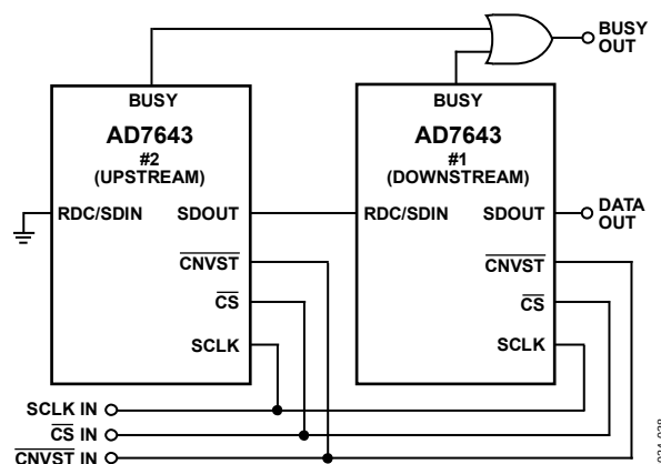
Figure 38. Two AD7643 Devices in a Daisy-Chain Configuration
