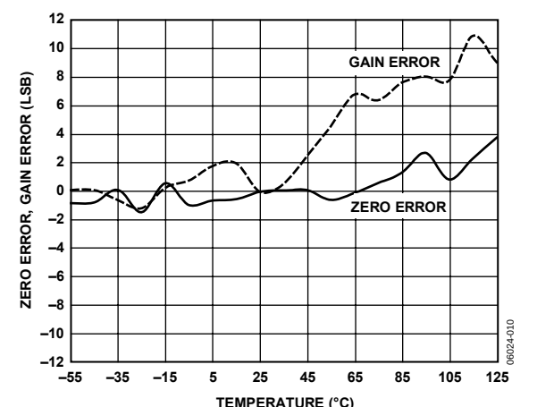
Figure 10. Zero Error, Gain Error vs. Temperature
