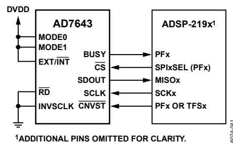
Figure 41. Interfacing the AD7643 to ADSP-219x
