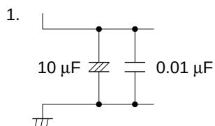
Figure 19.7 Example of Analog Input Protection Circuit
