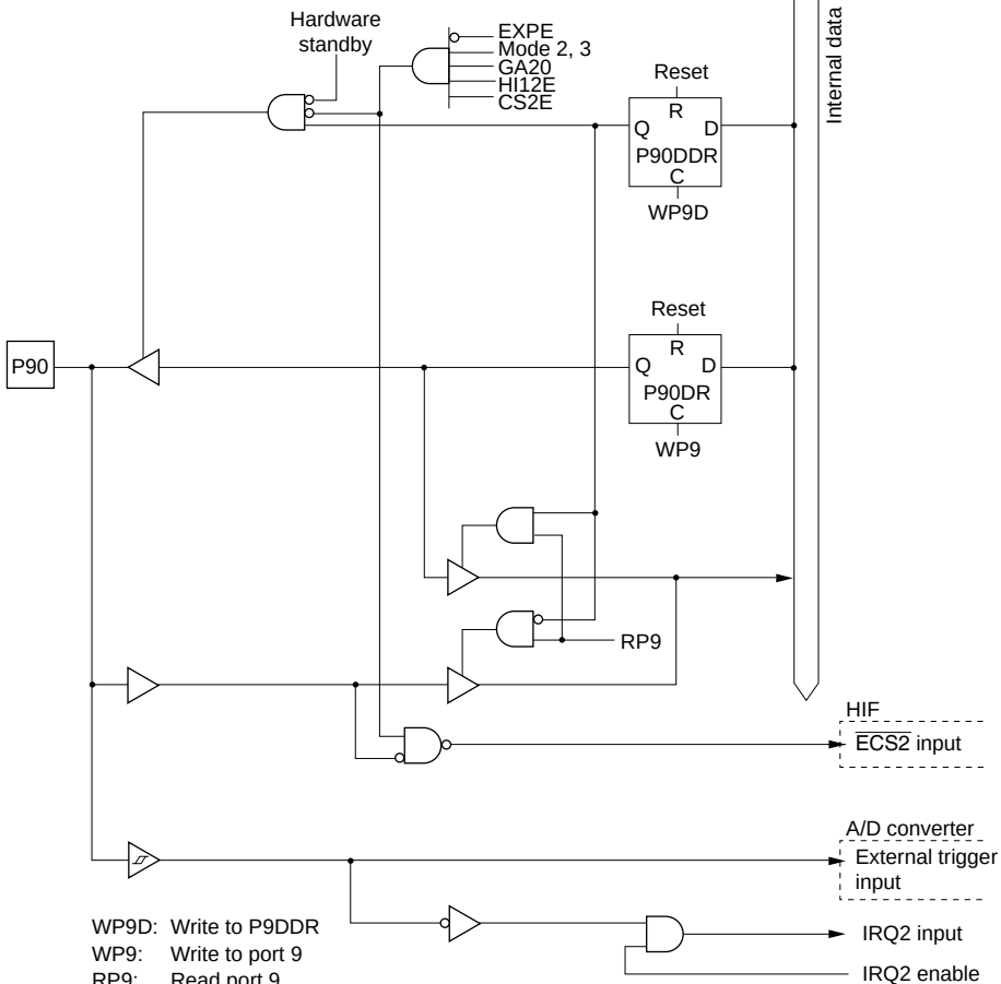
Figure C.29 Port 9 Block Diagram (Pin P90)
