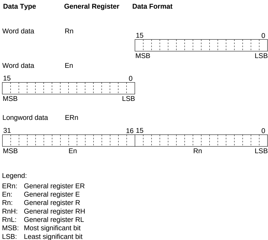
Figure 2.10 General Register Data Formats (cont)
