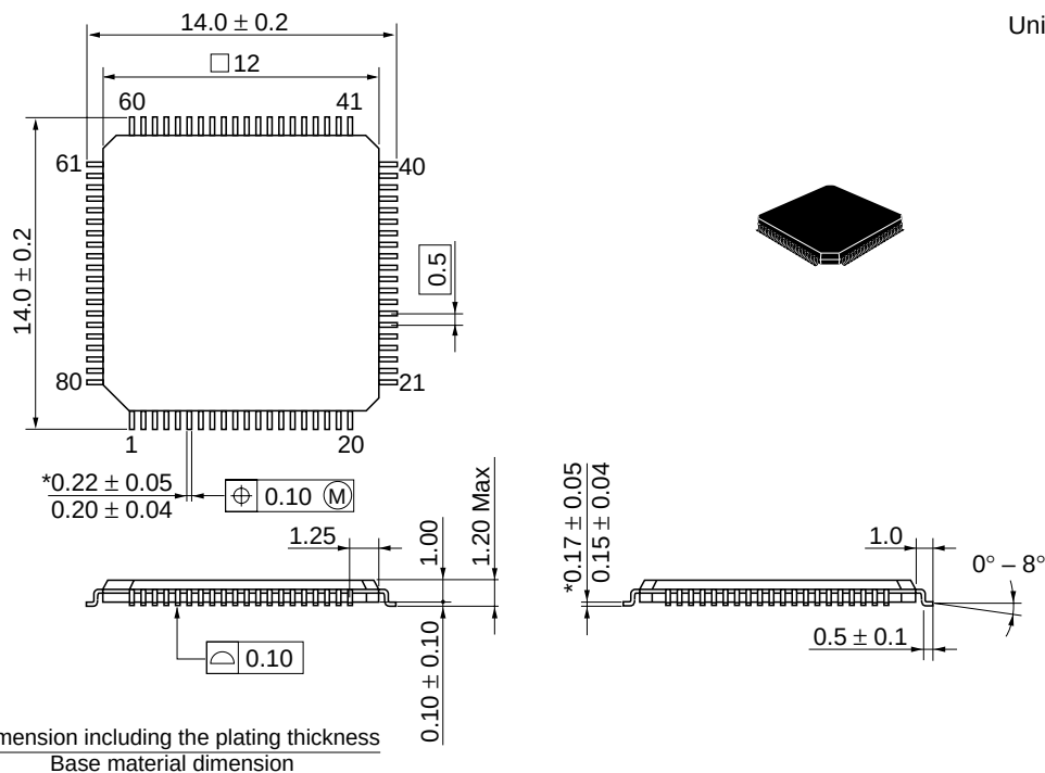
Figure G.2 Package Dimensions (TFP-80C)
