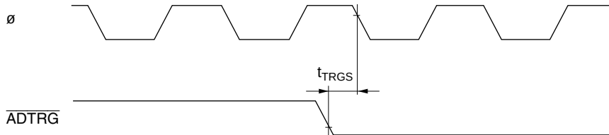
Figure 25.24 A/D Converter External Trigger Input Timing
