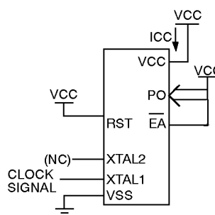
Figure 8. ICC Test Condition, Active Mode.
