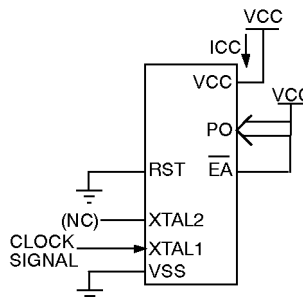
Figure 9. ICC Test Condition, Power Down Mode.
