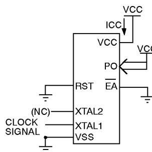
Figure 7. ICC Test Condition, Idle Mode.
