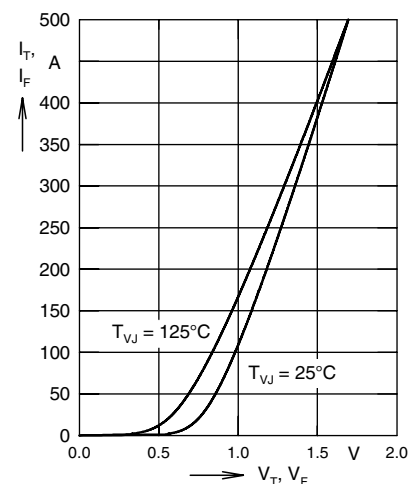
Fig 3: Forward current vs. voltage drop per thyristor/diode
