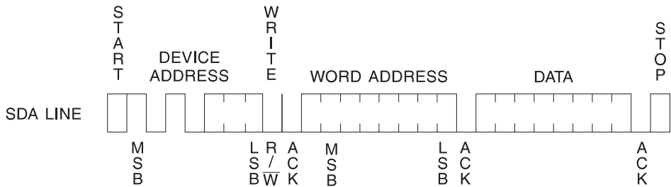
Figure 8-2. Byte Write
