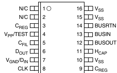
16-PIN SOIC PACKAGE
