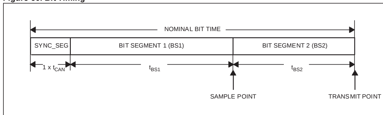
Figure 60. Bit Timing
