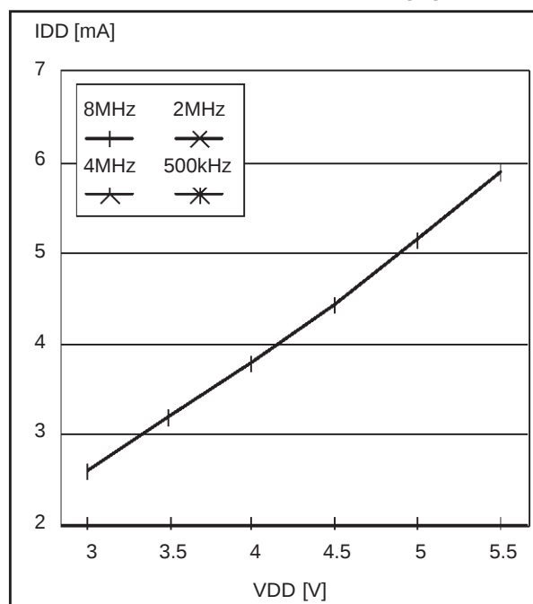
Figure 73. Typical I_{DD} in WAIT vs. f_{CPU}
