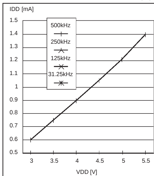
Figure 74. Typical I_{DD} in SLOW-WAIT vs. f_{CPU}
