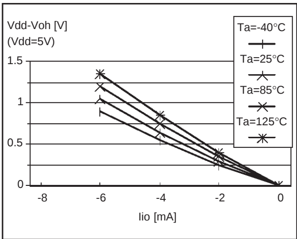
Figure 84. Typical V_{DD}-V_{OH} at V_{DD}=5V
