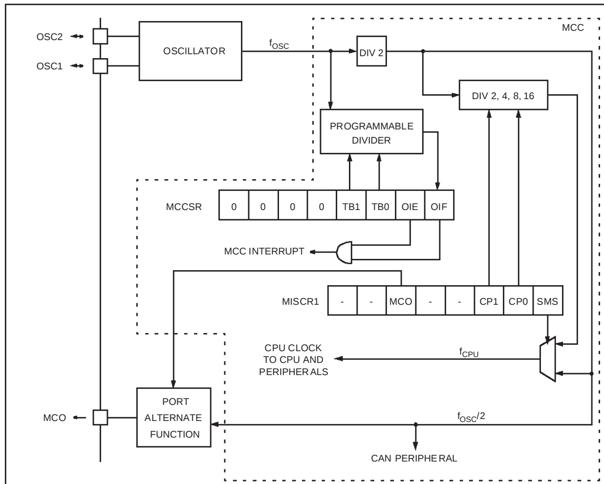
Figure 17. Main Clock Controller (MCC) Block Diagram
