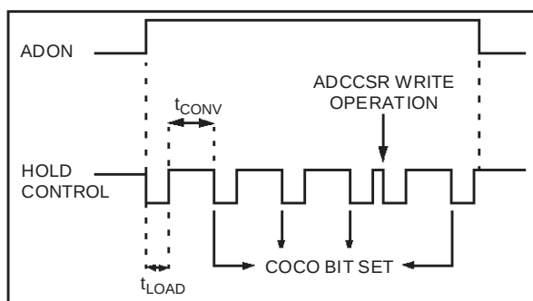
Figure 65. ADC Conversion Timings
