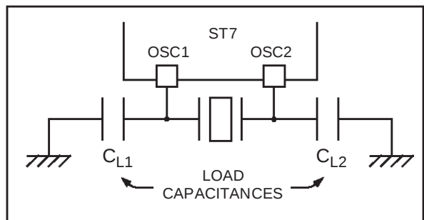
Figure 16. Crystal/Ceramic Resonator
