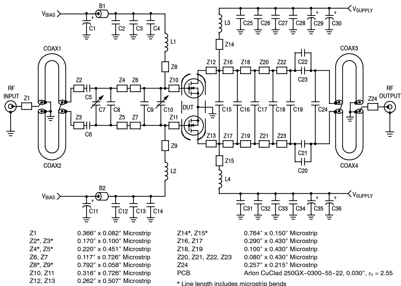
Figure 2. MRF6VP41KHR6(HSR6) Pulse Test Circuit Schematic — 450 MHz
