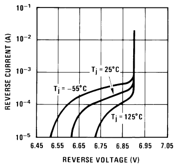
Reverse Characteristics
