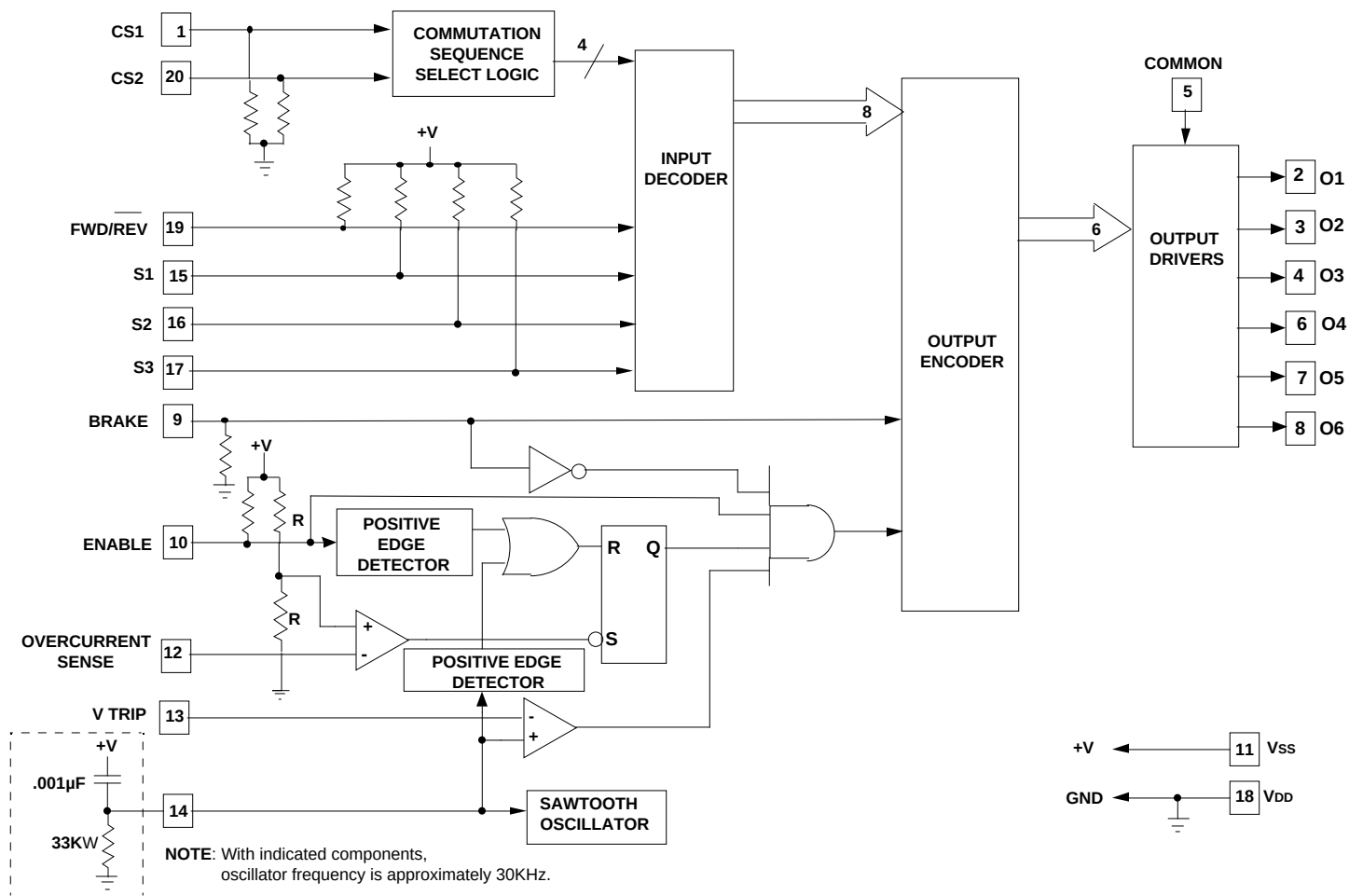
FIGURE 6. LS7260 AND LS7262 BLOCK DIAGRAM
