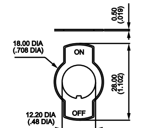
SWITCH PLATE ON-OFF U19 .480 I.D.
