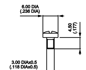
CONNECTING SCREW U03
