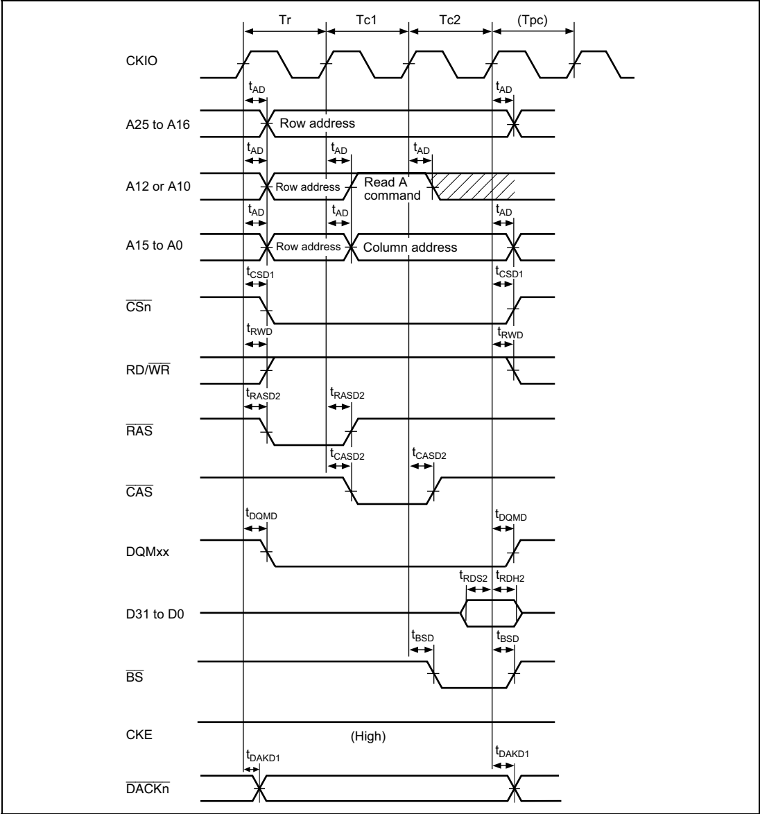
Figure 32.21 Synchronous DRAM Read Bus Cycle (RCD = 0, CAS Latency = 1, TPC = 0)
