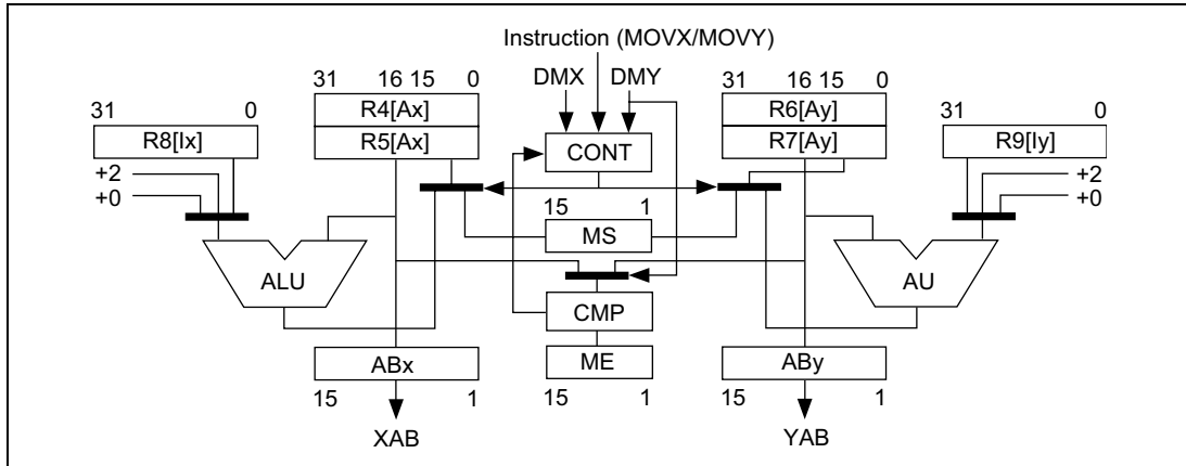
Figure 2.14 Modulo Addressing
