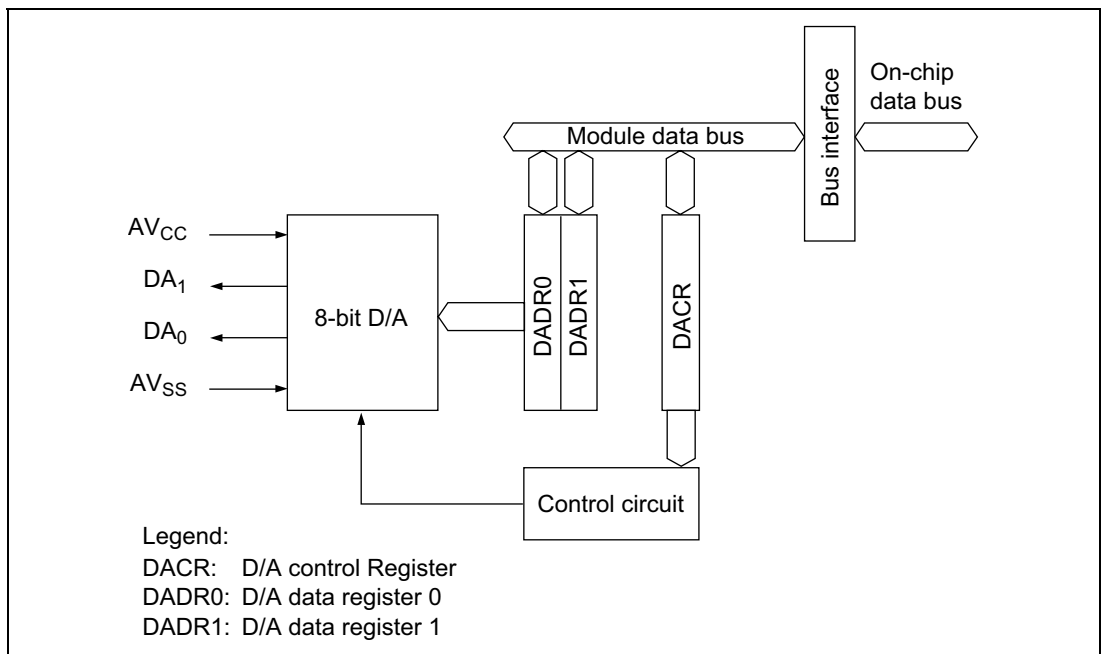
Figure 29.1 D/A Converter Block Diagram
