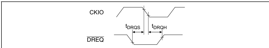
Figure 32.43 \overline{DREQ} Input Timing
