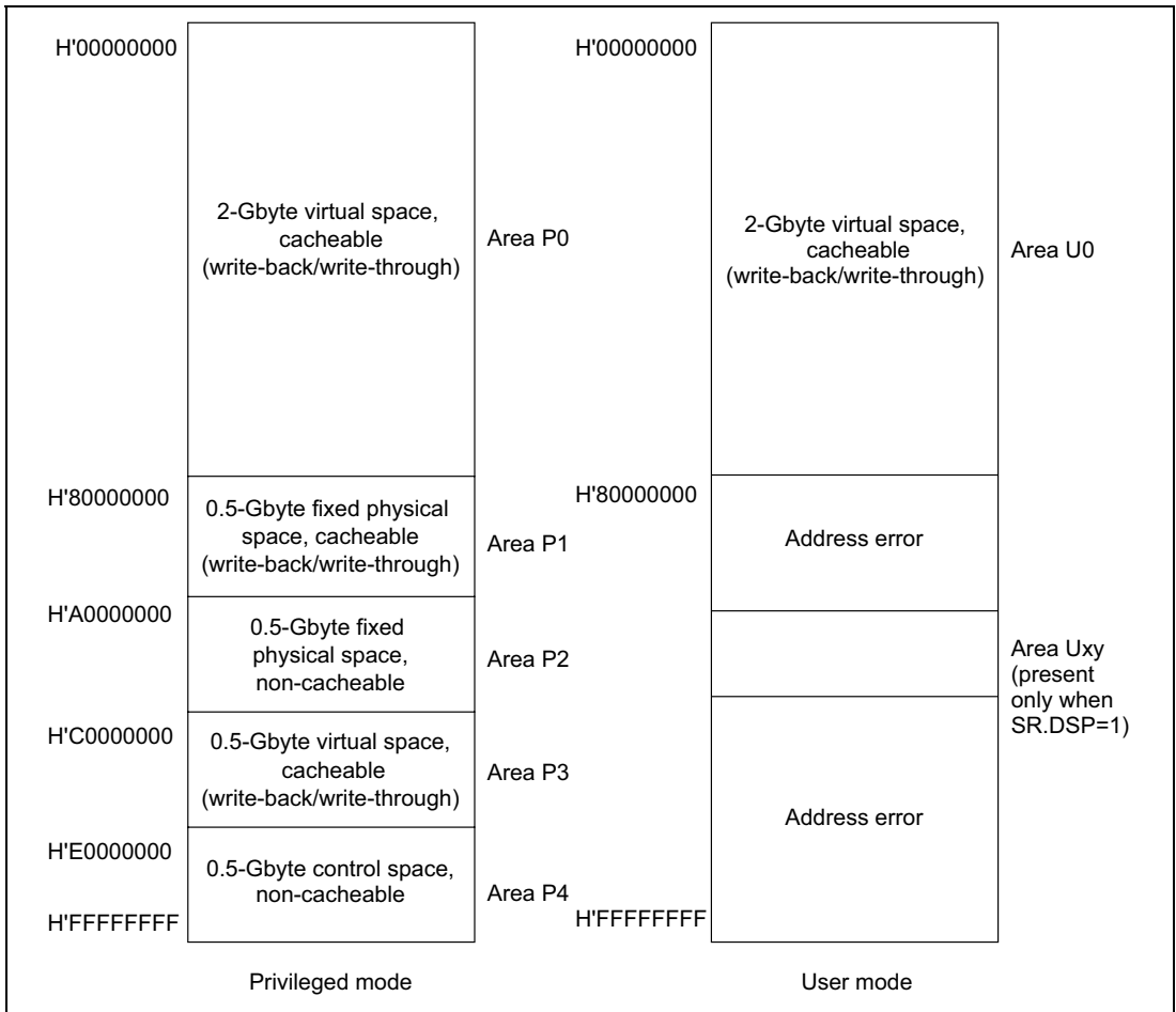
Figure 3.2 Logical Address Space Mapping
