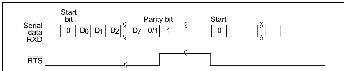
Figure 19.11 Example of Operation Using Modem Control ( \overline{\text{RTS}} )
