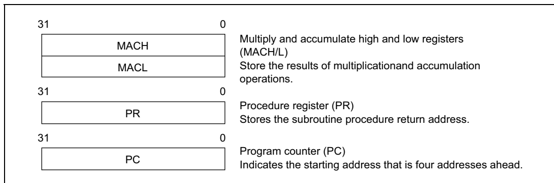
Figure 2.6 System Registers
