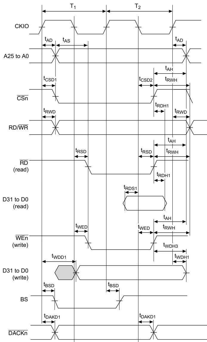
Figure 32.15 Basic Bus Cycle (No Wait)
