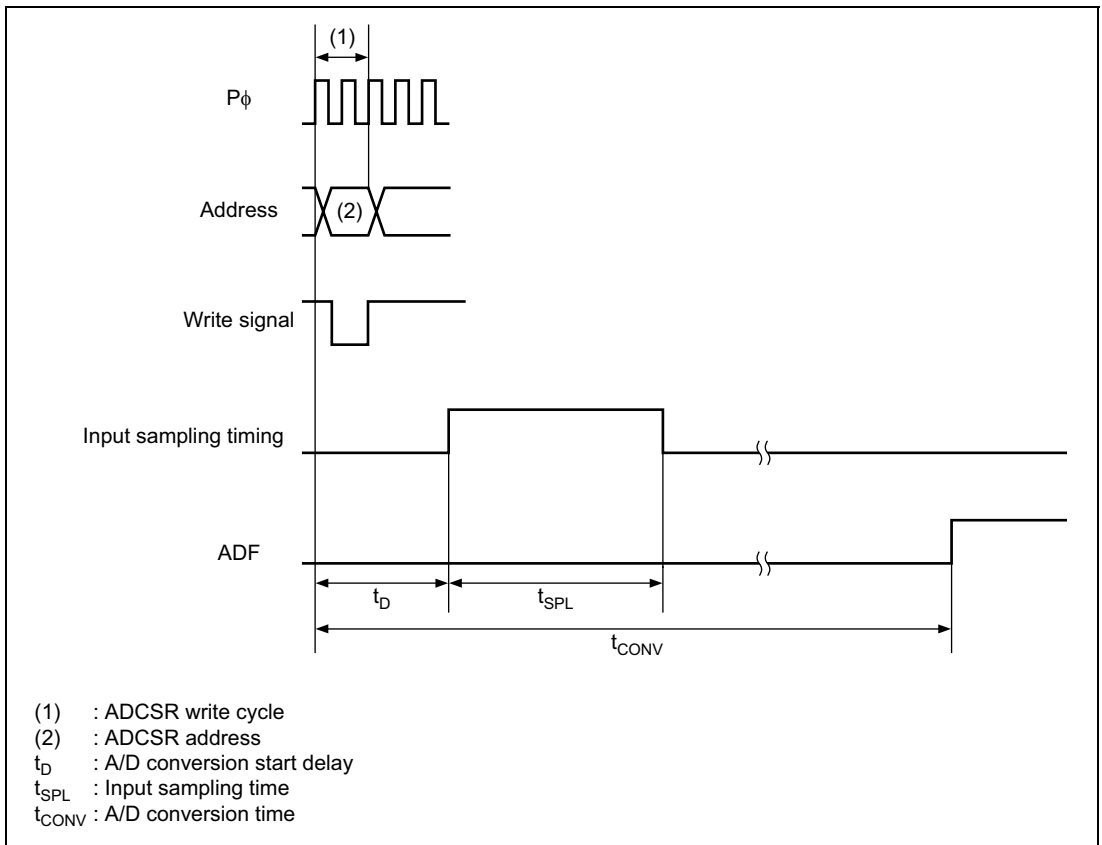
Figure 28.6 A/D Conversion Timing
