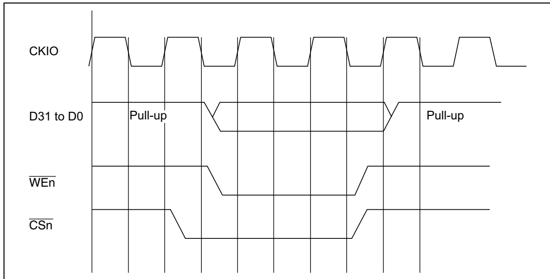
Figure 12.36 Pins D31 to D0 Pull-Up Timing (Write Cycle)
