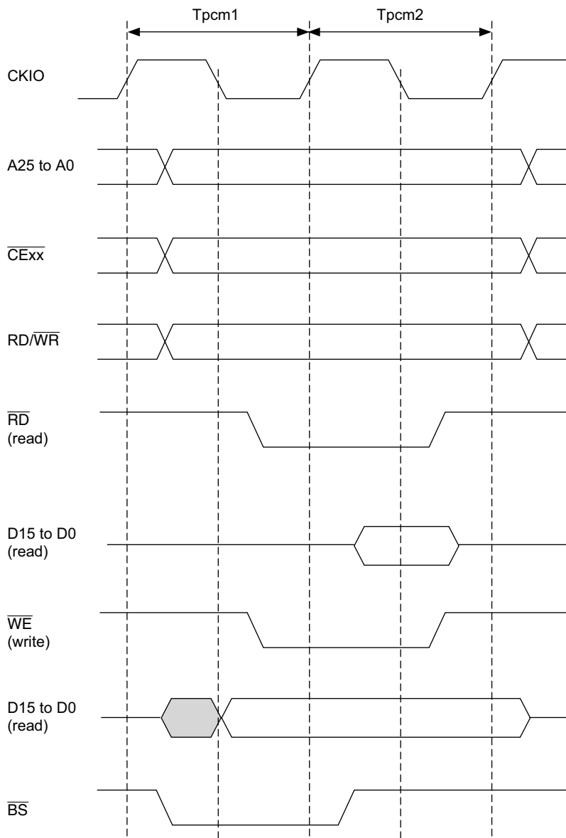
Figure 12.25 Basic Timing for PCMCIA Memory Card Interface
