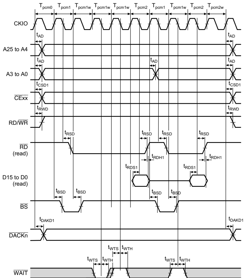
Figure 32.35 PCMCIA Memory Bus Cycle (Burst Read, TED = 1, TEH = 1, Two Waits, Burst Pitch = 3, WAITSEL = 1)
