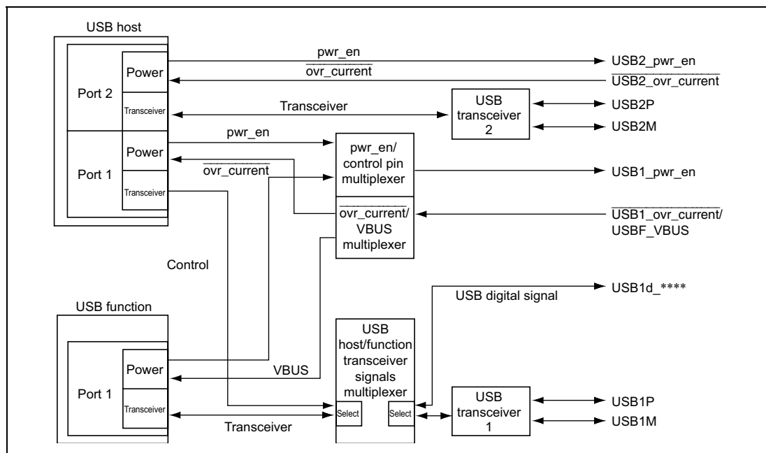
Figure 22.1 Block Diagram of USB PIN Multiplexer
