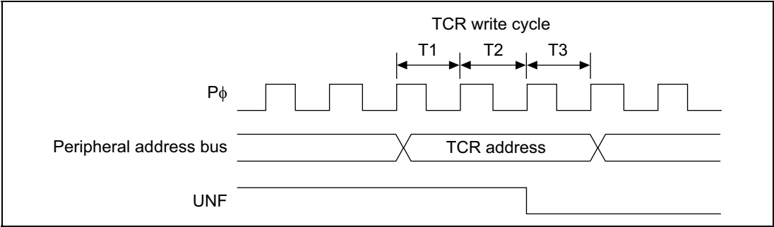
Figure 15.7 Status Flag Clear Timing
