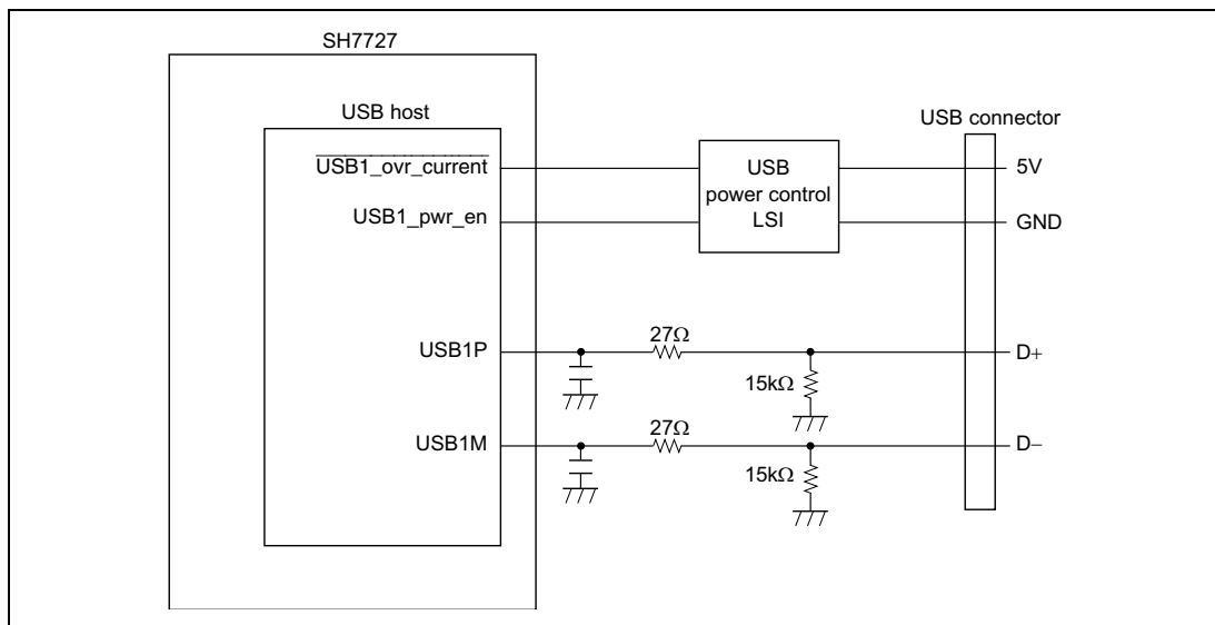
Figure 22.6 Example 1 of Transceiver Connection for USB Host Controller (On-chip transceiver is used)
