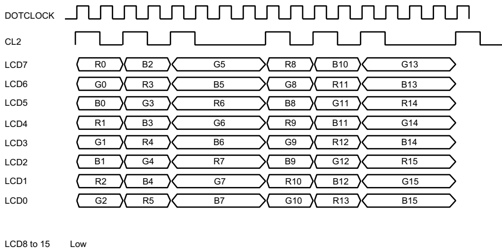
Figure 25.11 Clock and LCD Data Signal Example
