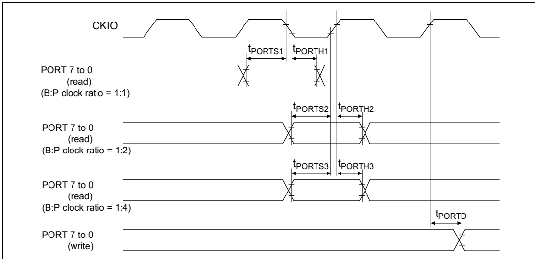
Figure 32.42 I/O Port Timing
