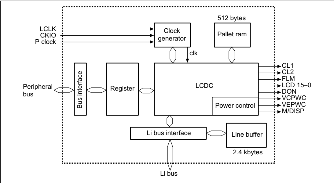
Figure 25.1 Block Diagram
