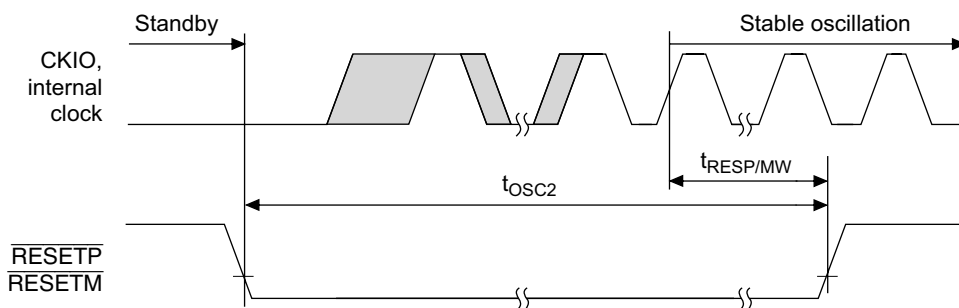
Figure 32.4 Power-on Oscillation Settling Time
