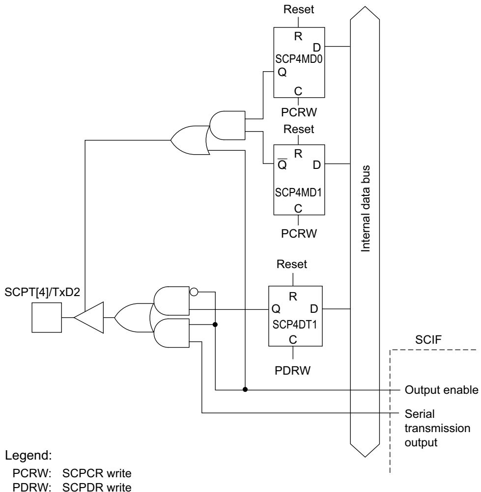
Figure 19.2 SCPT[4]/TxD2 Pin
