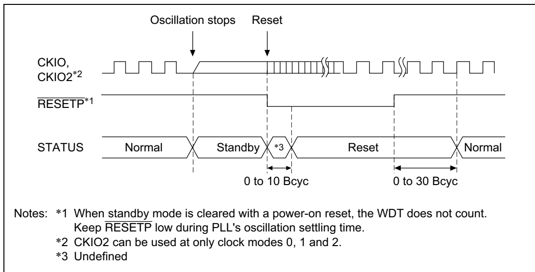
Figure 9.5 Standby to Power-On Reset STATUS Output
