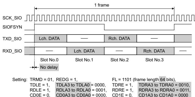
Figure 20.17 Transmit or Receive Timing (16 bits stereo—2)
