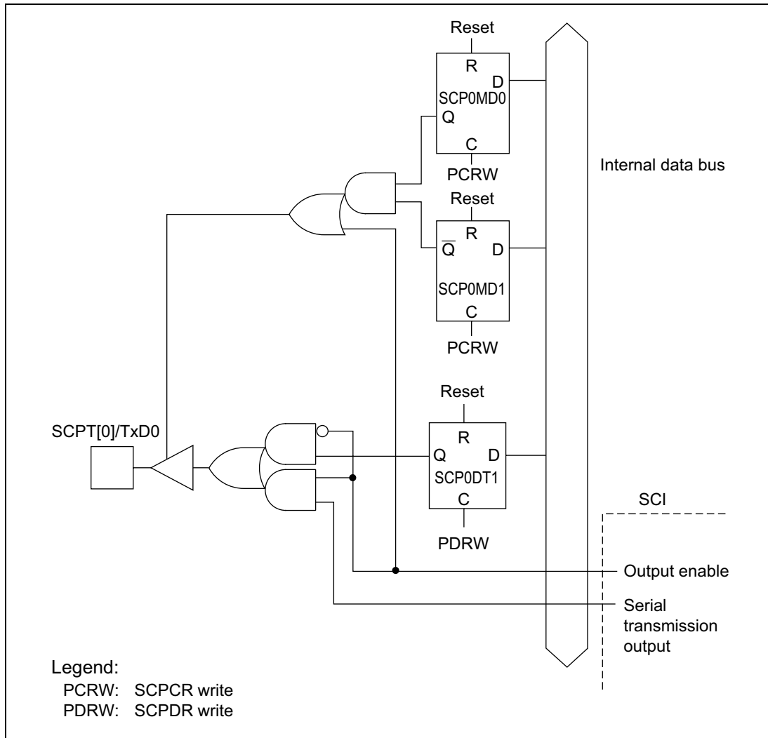
Figure 17.3 SCPT[0]/TxD0 Pin
