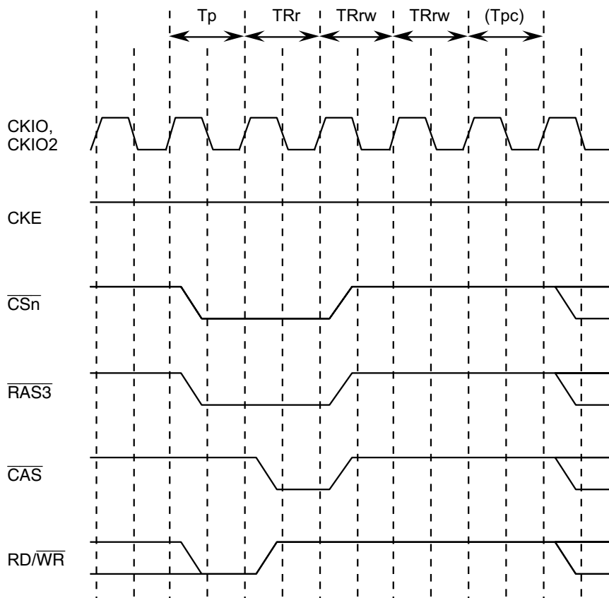
Figure 12.19 Synchronous DRAM Auto-Refresh Timing
