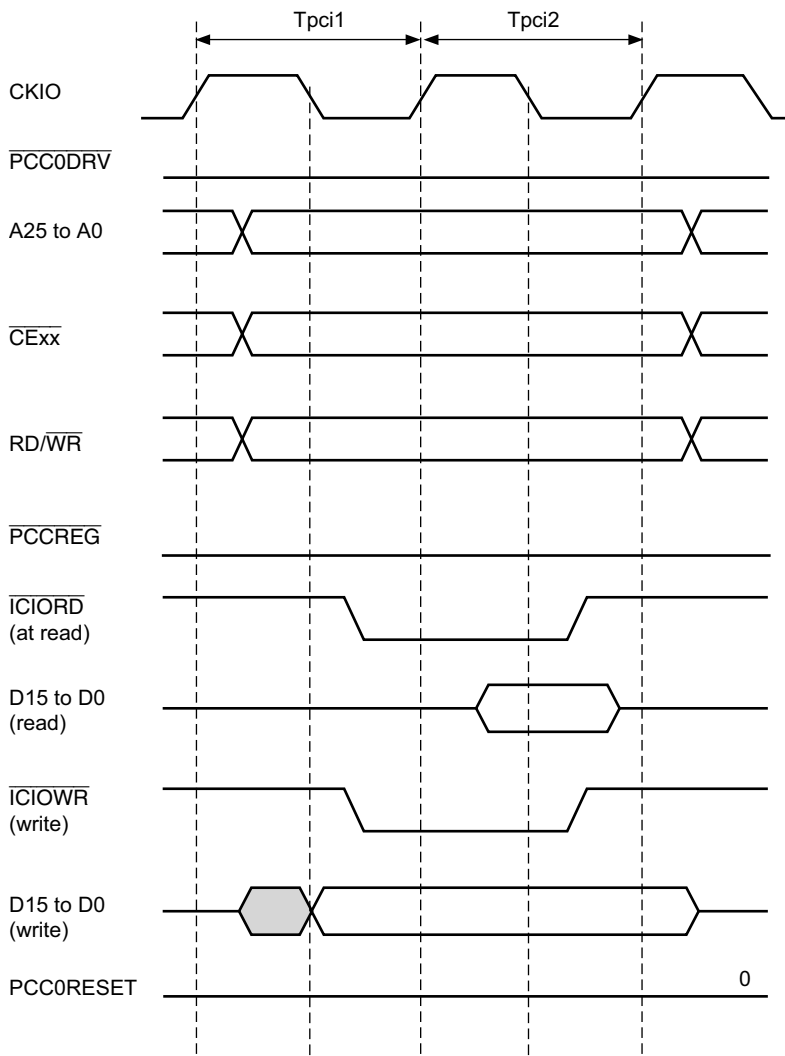
Figure 30.7 PCMCIA I/O Card Interface Basic Timing
