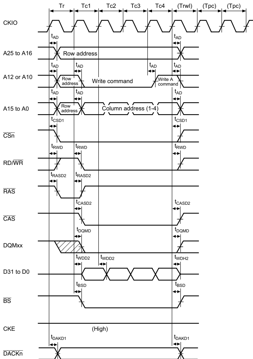
Figure 32.27 Synchronous DRAM Write Bus Cycle (Burst Mode (Single Write x 4), RCD = 0, TPC = 1, TRWL = 0)
