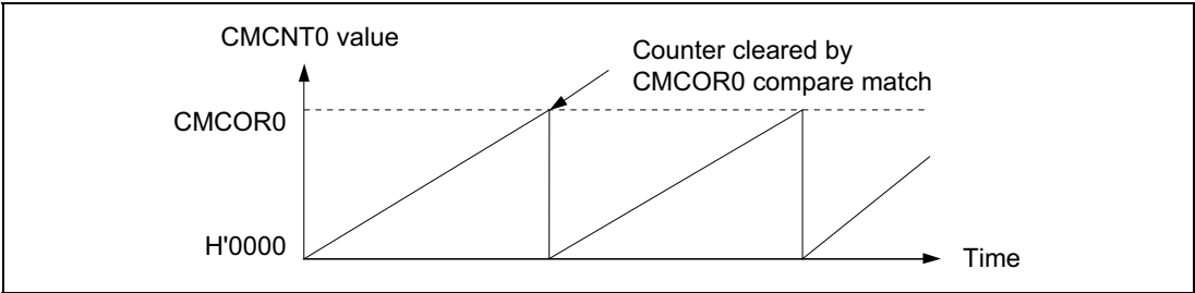
Figure 14.27 Counter Operation
