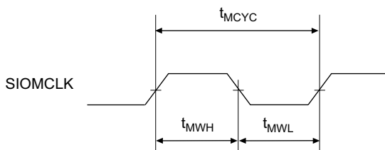
Figure 32.50 SIOMCLK Input Timing
