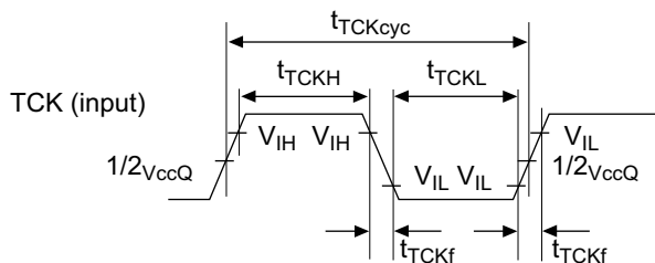
Figure 32.45 TCK Input Timing
