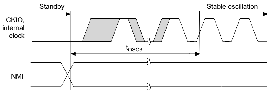
Figure 32.5 Oscillation Settling Time at Standby Return (Return by Reset)
