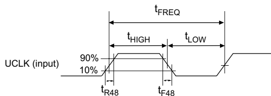
Figure 32.56 USB Clock Timing
