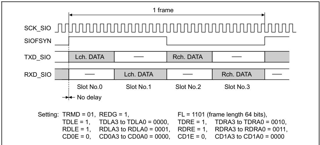
Figure 20.17 Transmit or Receive Timing (16 bits stereo—2)
