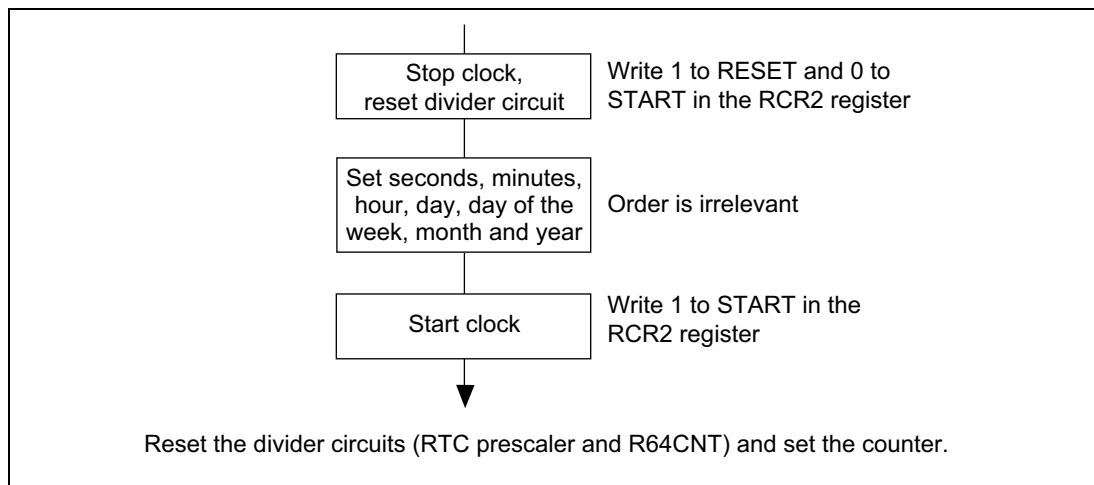
Figure 16.2 Setting the Time
