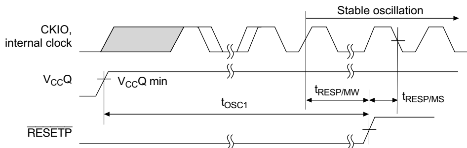
Figure 32.4 Power-on Oscillation Settling Time
