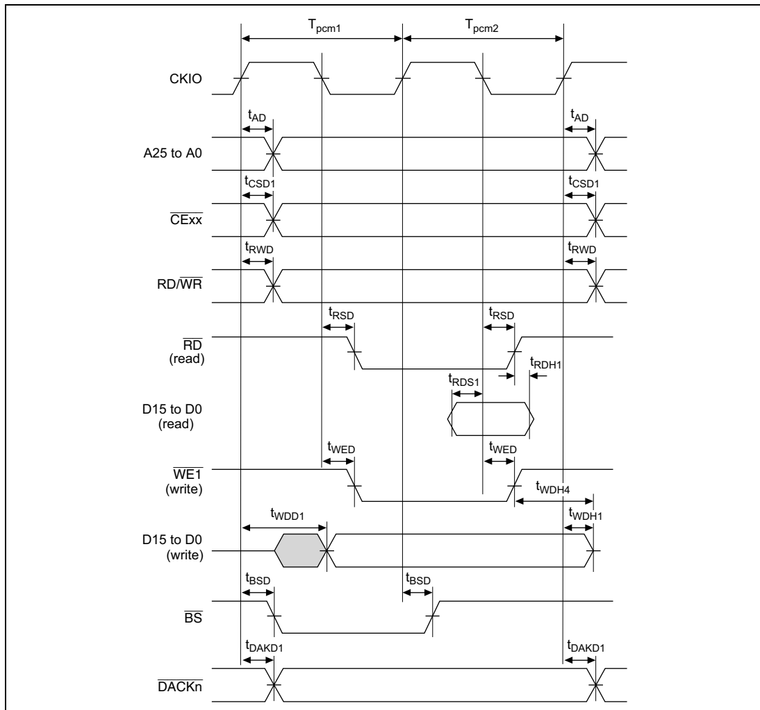
Figure 32.32 PCMCIA Memory Bus Cycle (TED = 0, TEH = 0, No Wait)
