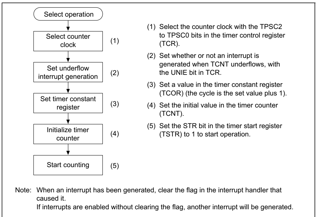
Figure 15.2 Setting the Count Operation
