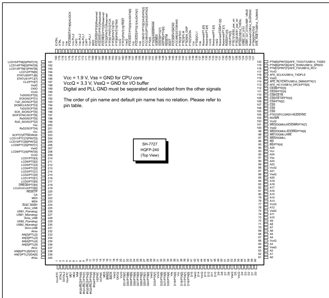
Figure 1.2 Pin Arrangement (FP-240B)
