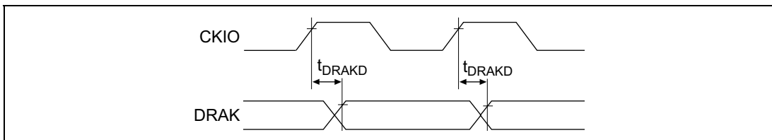
Figure 32.44 DRAK Output Timing
