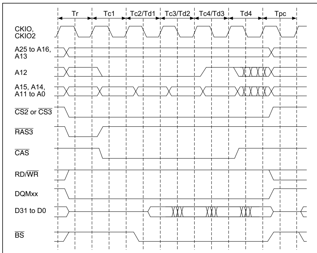
Figure 12.13 Basic Timing for Synchronous DRAM Burst Read
