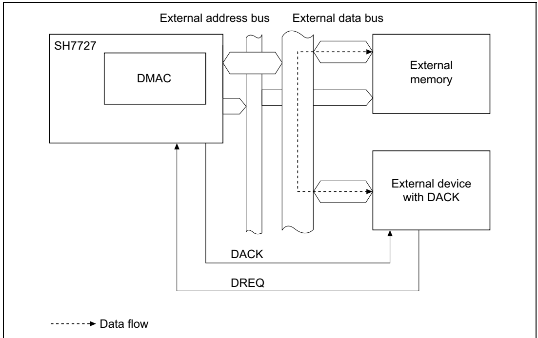
Figure 14.11 Data Flow in Single Address Mode
