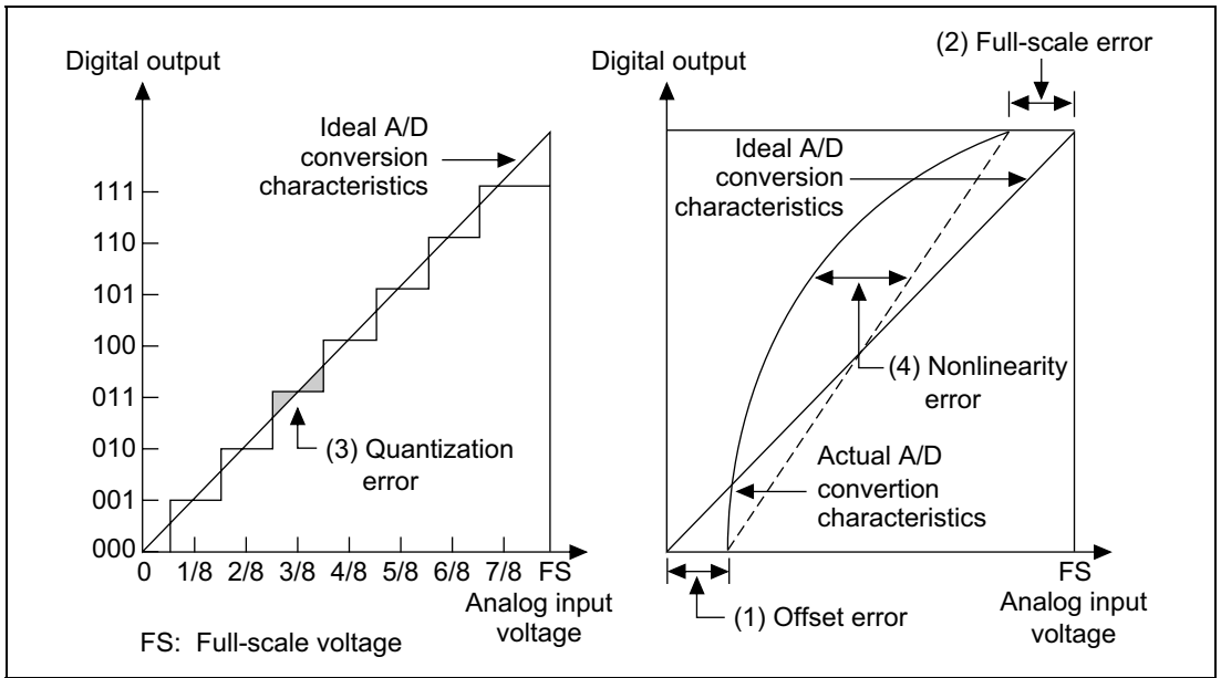
Figure 28.8 Definitions of A/D Conversion Accuracy
