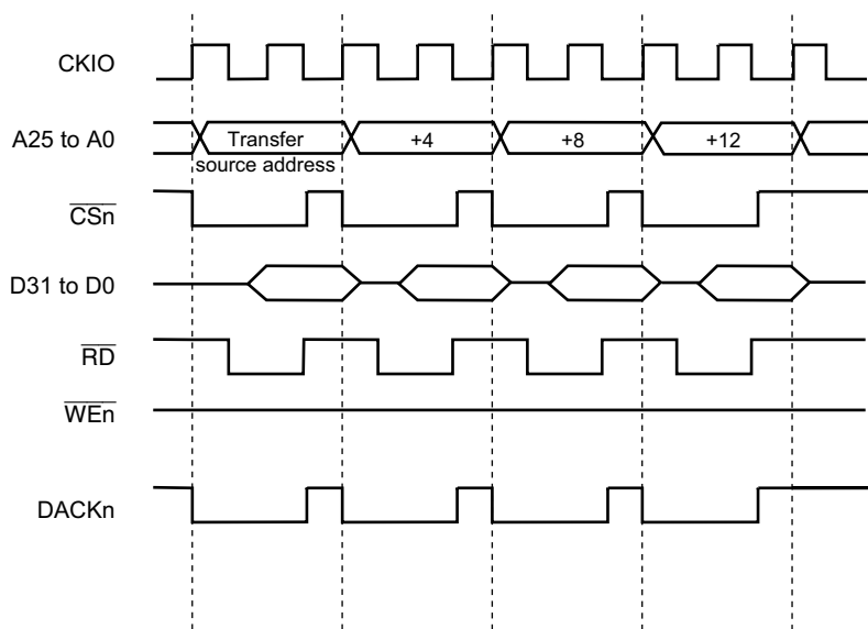
Figure 14.13 Example of DMA Transfer Timing in Single Address Mode (External Memory Space (Ordinary Memory) → External Device with DACK)
