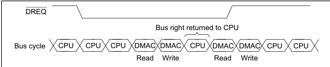
Figure 14.14 Transfer Example in Cycle-Steal Mode
