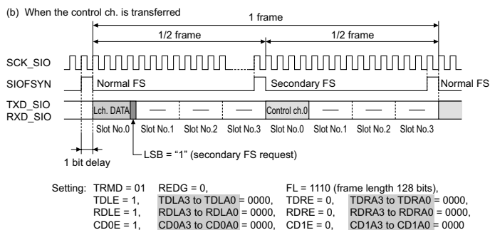
Figure 20.19 Transmit or Receive Timing (16 bits monaural—2)
