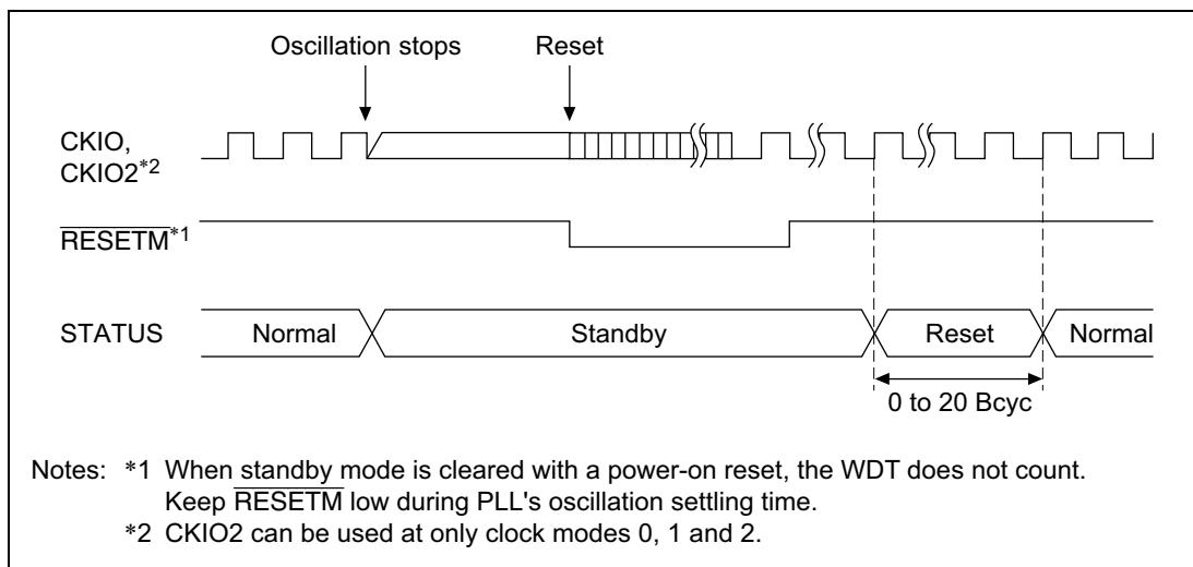
Figure 9.6 Standby to Manual Reset STATUS Output
