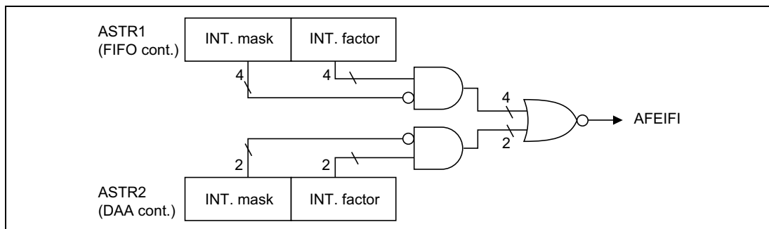
Figure 21.4 Interrupt Generator
