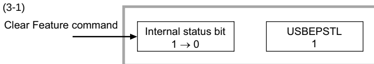
Figure 23.13 Forcible Stall by Application
