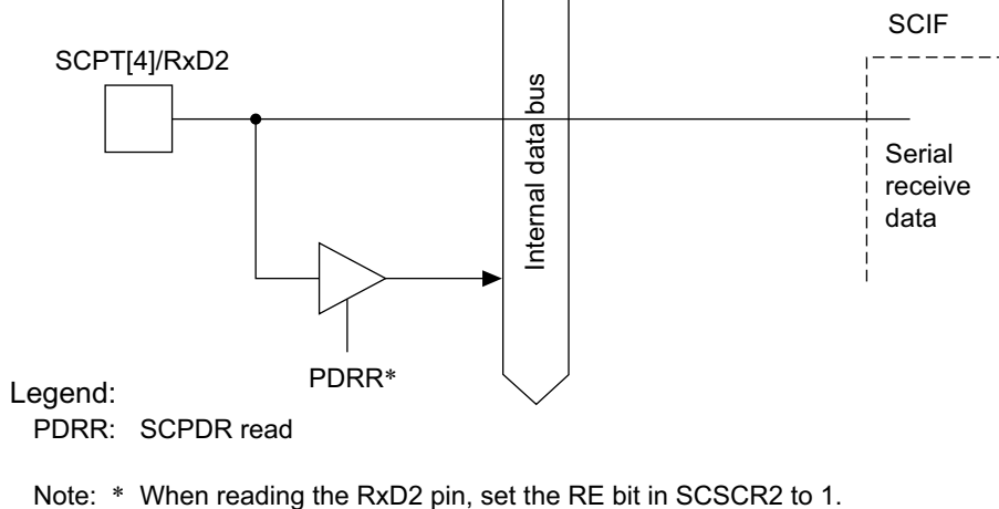
Figure 19.3 SCPT[4]/RxD2 Pin
