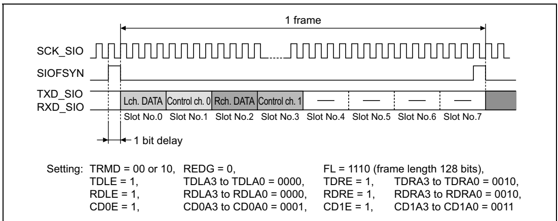
Figure 20.18 Transmit or Receive Timing (16 bits stereo—3)
