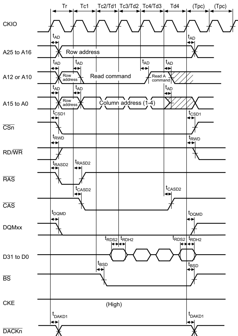
Figure 32.23 Synchronous DRAM Read Bus Cycle (Burst Read (Single Read \times 4), RCD = 0, CAS Latency = 1, TPC = 1)
