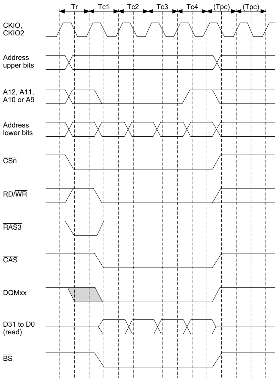
Figure 12.16 Basic Timing for Synchronous DRAM Burst Write
