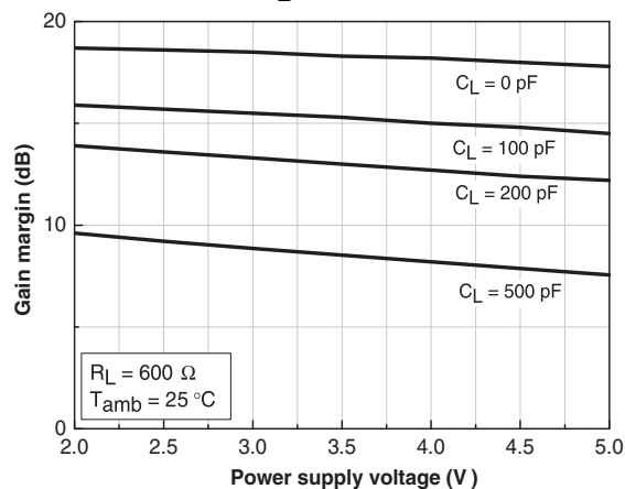
Figure 26. Gain margin vs. supply voltage ( R_L = 600\ \Omega )
