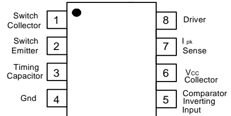
PDIP-8 ( Top View )
