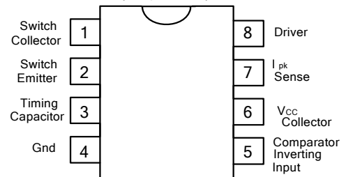
PDIP-8 ( Top View )
