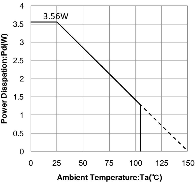
Fig.40 Power Dissipation
