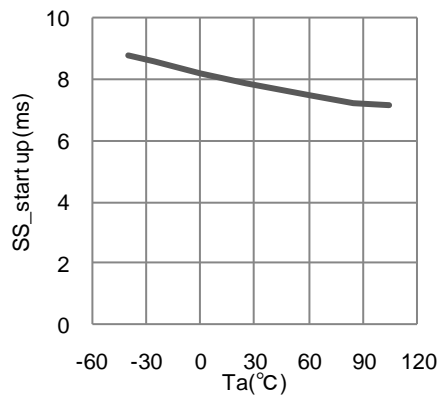
Fig.10. Soft start vs temp
