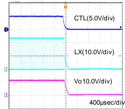
Fig.25 Stop (Rload=2.5Ω)
