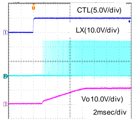
Fig.23 Start-up
