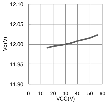
Fig.19 Line Regulation
