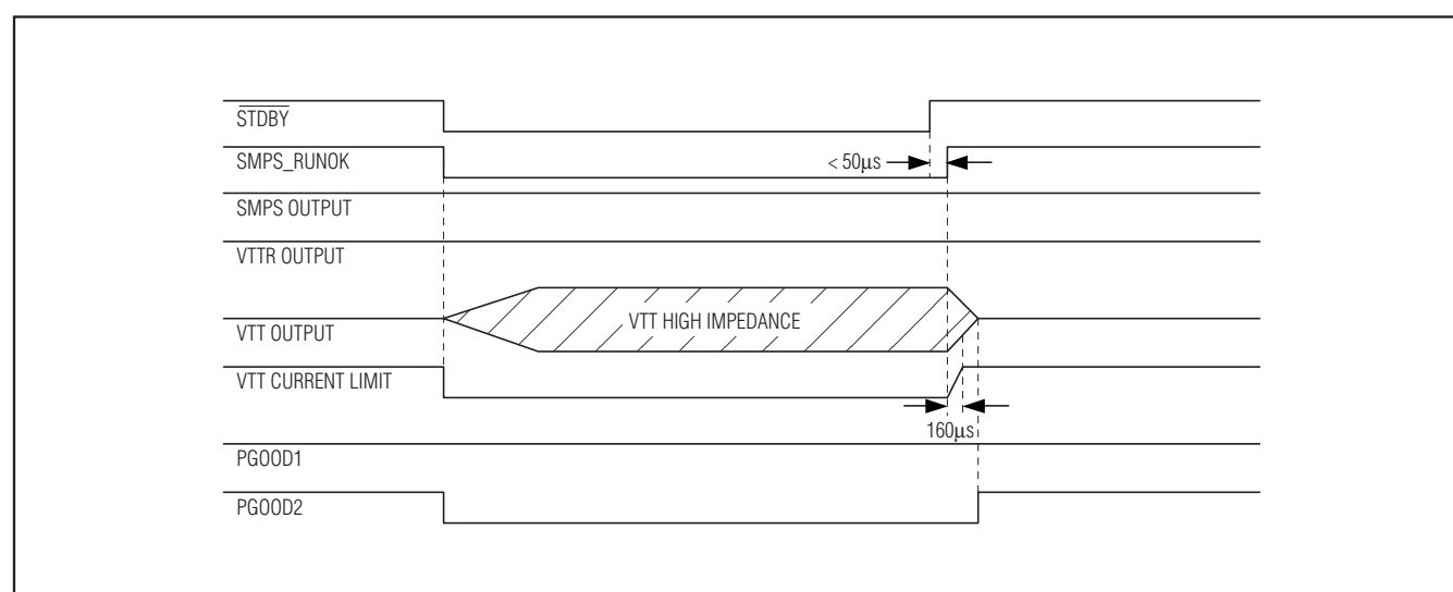
Figure 4. MAX17000 Standby Mode Timing
