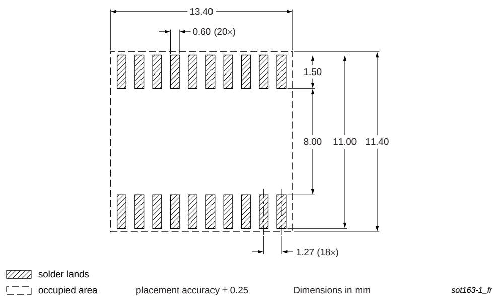
Fig 43. Reflow soldering of the SO20 package
