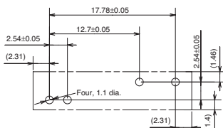
Mounting Holes (Bottom View)
