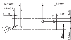
Mounting Holes (Bottom View)
