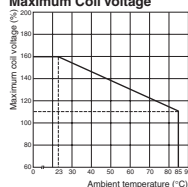
Ambient Temperature vs. Maximum Coil Voltage
