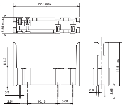
Connecting Socket P6DS-04P
