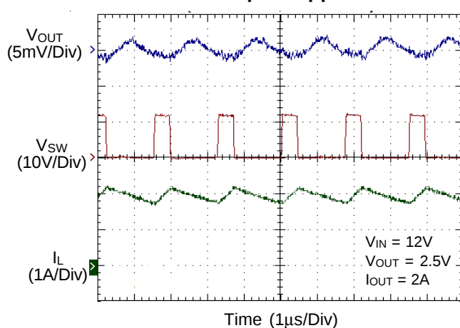
Output Ripple
