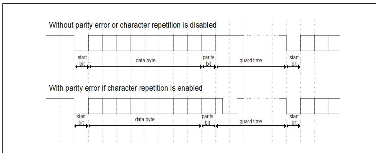
FIGURE 13-2: T=0 MODE CHARACTER TRANSMISSION AND REPETITION DIAGRAM
