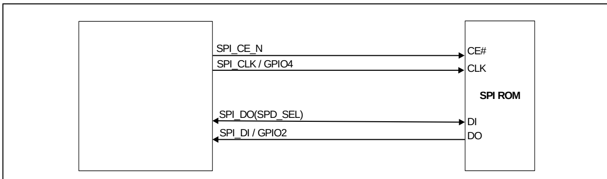
FIGURE 2-1: SPI ROM Connection
