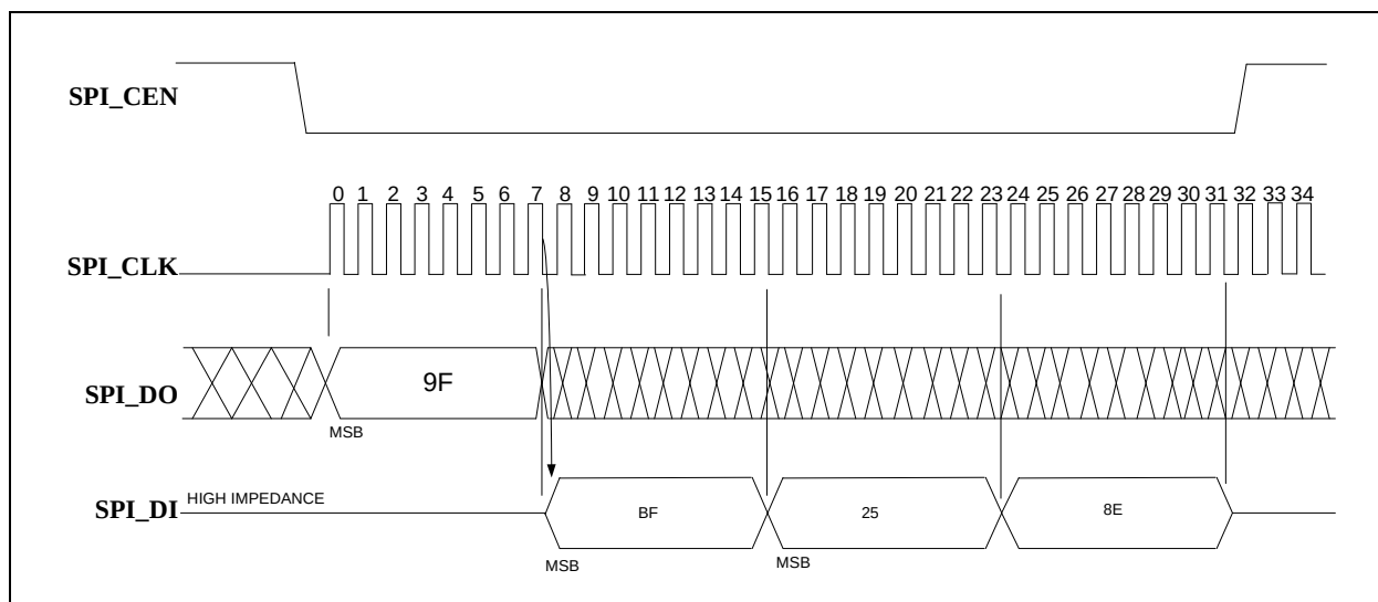
FIGURE 12-6: SPI JEDEC-ID SEQUENCE
