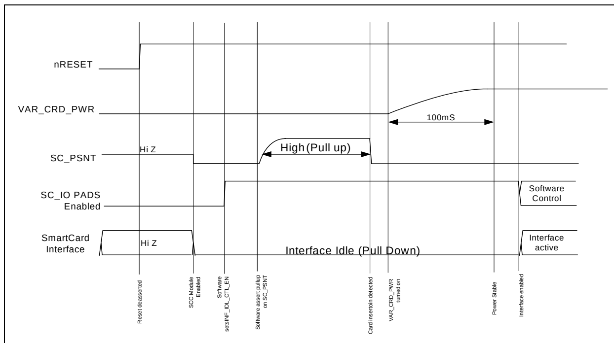
FIGURE 13-12: SMARTCARD POWERUP
