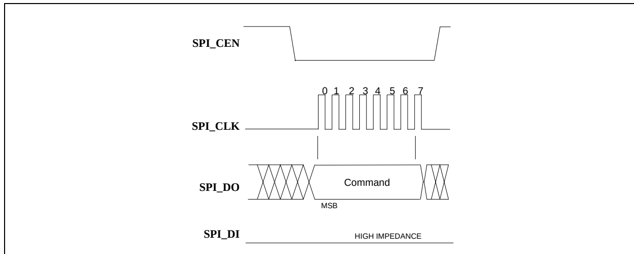
FIGURE 12-5: SPI COMMAND ONLY SEQUENCE
