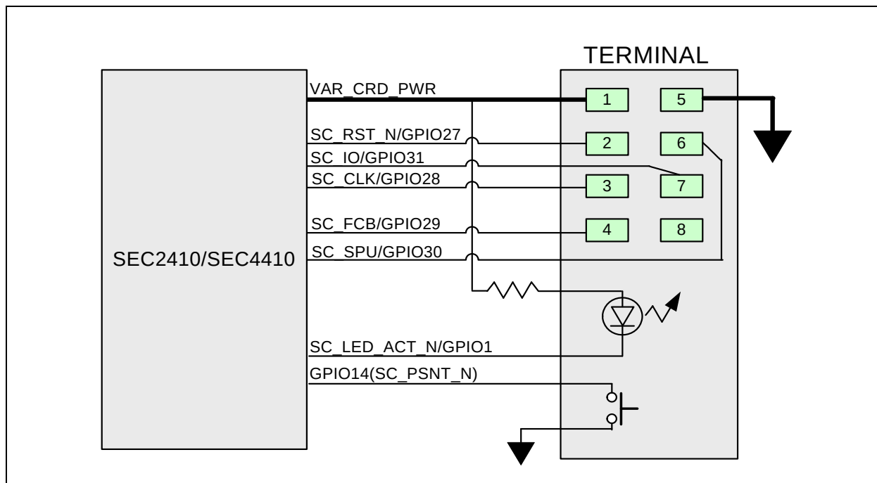
FIGURE 13-1: SMARTCARD INTERCONNECT
