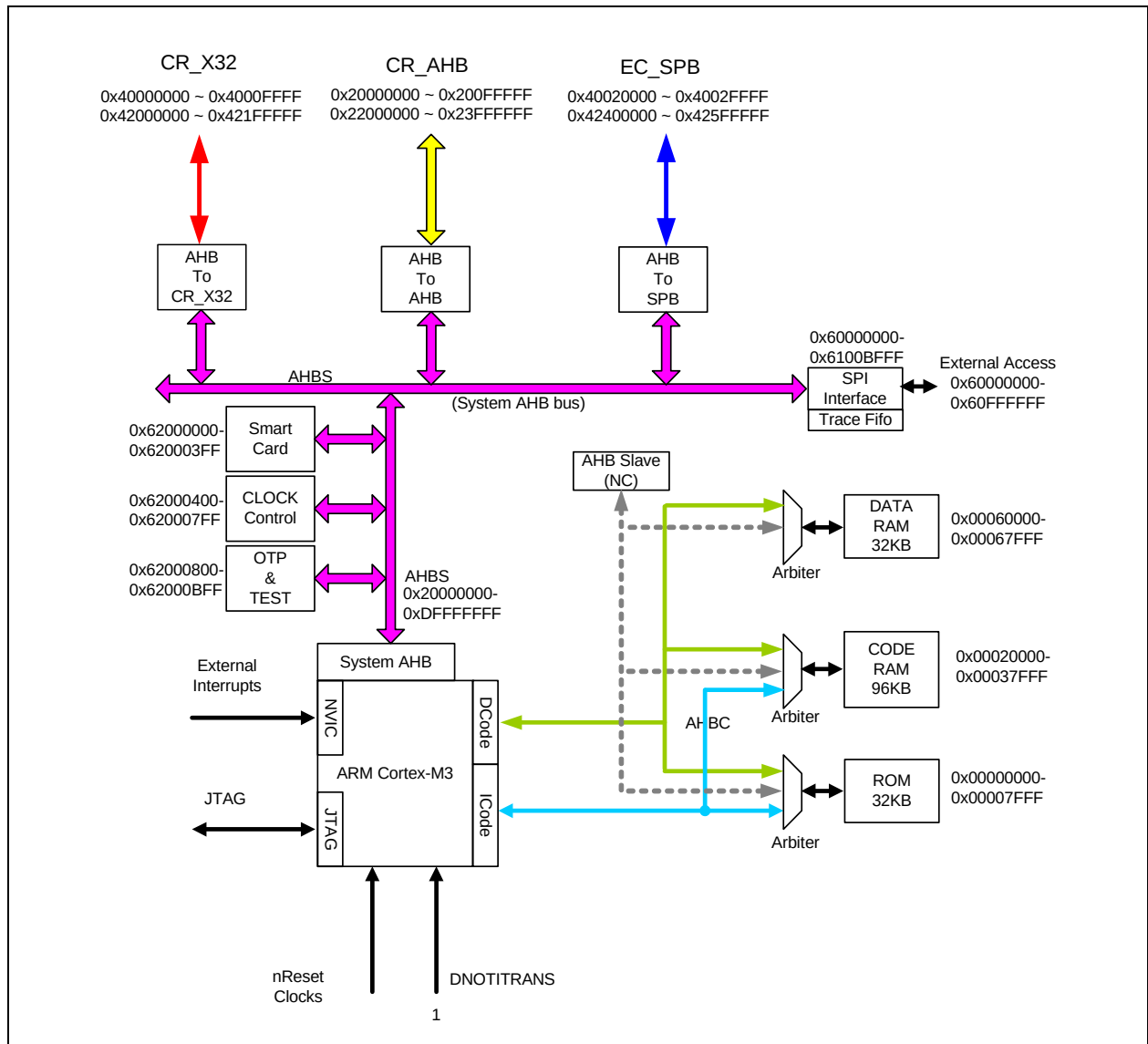
FIGURE 7-1: BUS ADDRESSES
