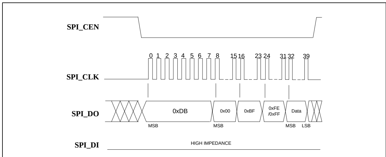
FIGURE 12-4: SPI BYTE PROGRAM
