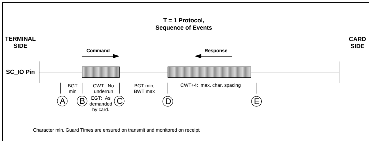
FIGURE 13-3: T=1 EVENTS
