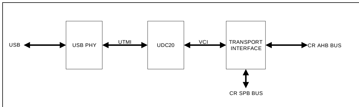
FIGURE 16-1: USB INTERFACE
